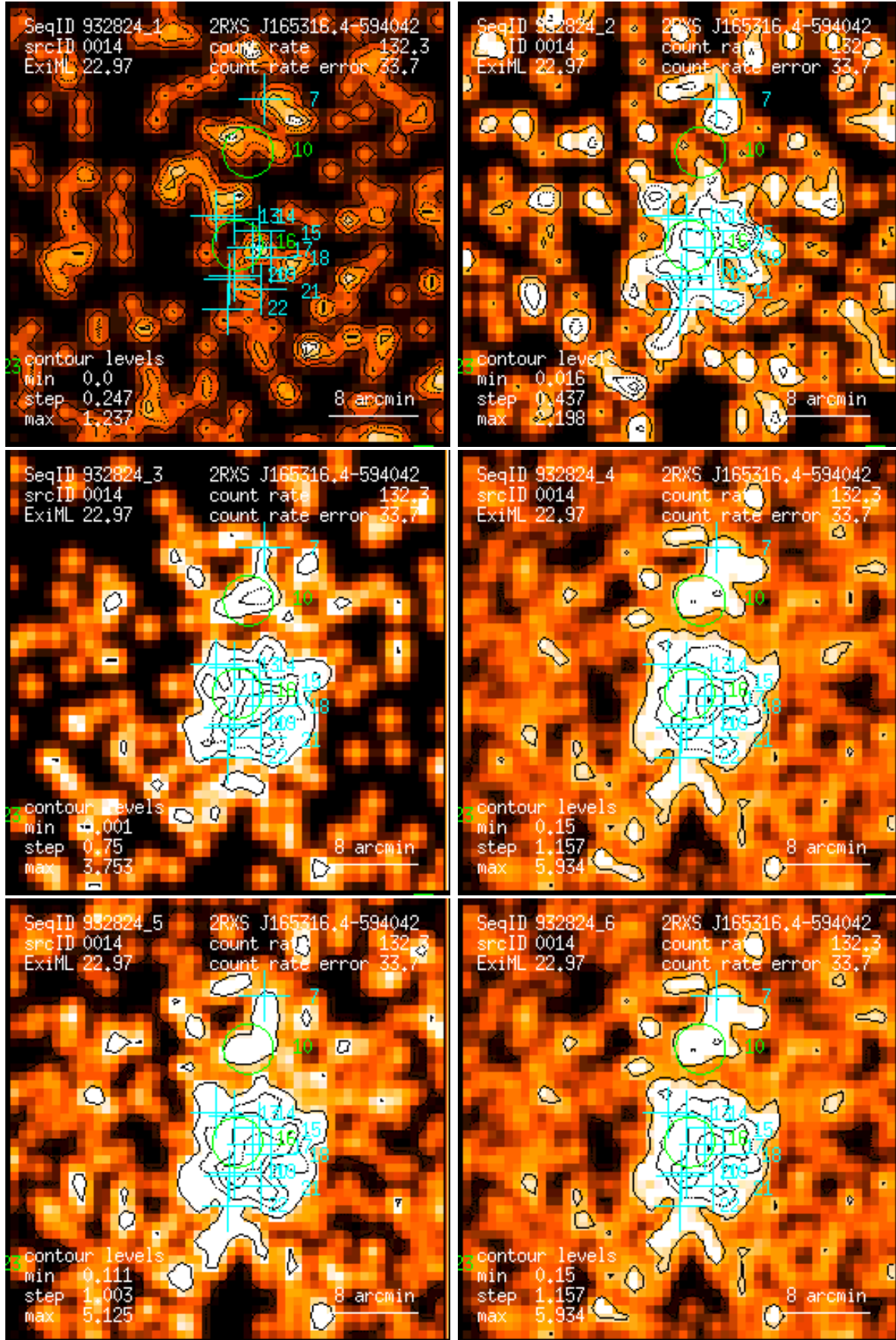
Figure 14: RASS 932824: detection 0014: band rate images, Gaussian filter: (1) PSPC channels 11 – 41, (2) 52 – 90, (3) 91 – 201, (4) 11 – 235, (5) 52 – 201, (6) 11 – 201. Broad band rates in counts/ks. Band rate contour levels in counts/ks/arcmin 2 .
