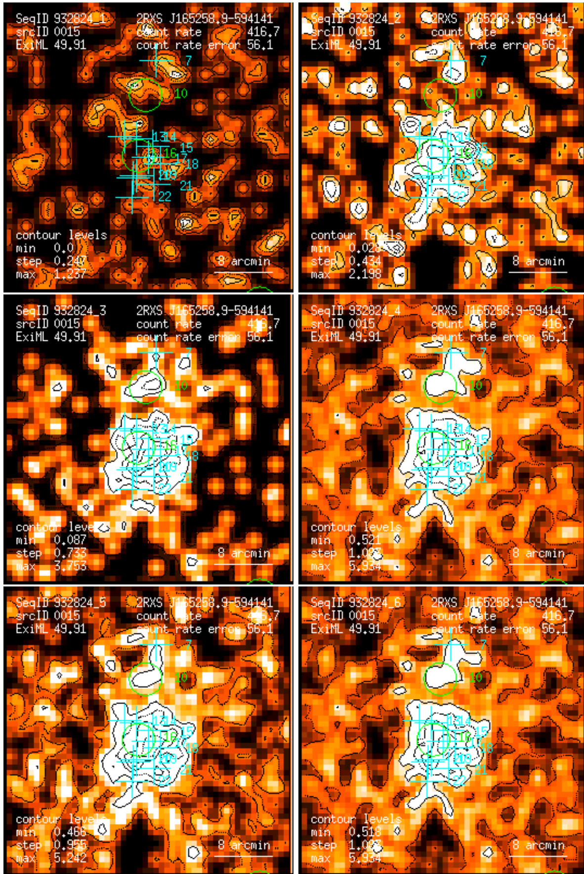
Figure 15: RASS 932824: detection 0015: band rate images, Gaussian filter: (1) PSPC channels 11 – 41, (2) 52 – 90, (3) 91 – 201, (4) 11 – 235, (5) 52 – 201, (6) 11 – 201. Broad band rates in counts/ks. Band rate contour levels in counts/ks/arcmin 2 .
