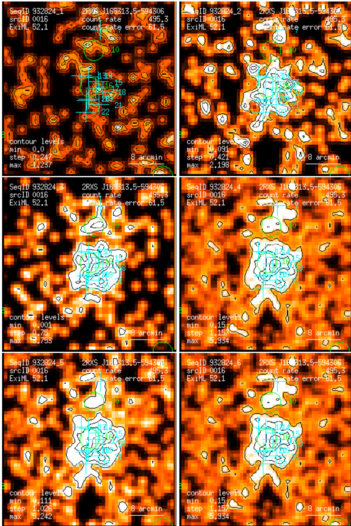
Figure 16: RASS 932824: detection 0016: band rate images, Gaussian filter: (1) PSPC channels 11 – 41, (2) 52 – 90, (3) 91 – 201, (4) 11 – 235, (5) 52 – 201, (6) 11 – 201. Broad band rates in counts/ks. Band rate contour levels in counts/ks/arcmin 2 .
