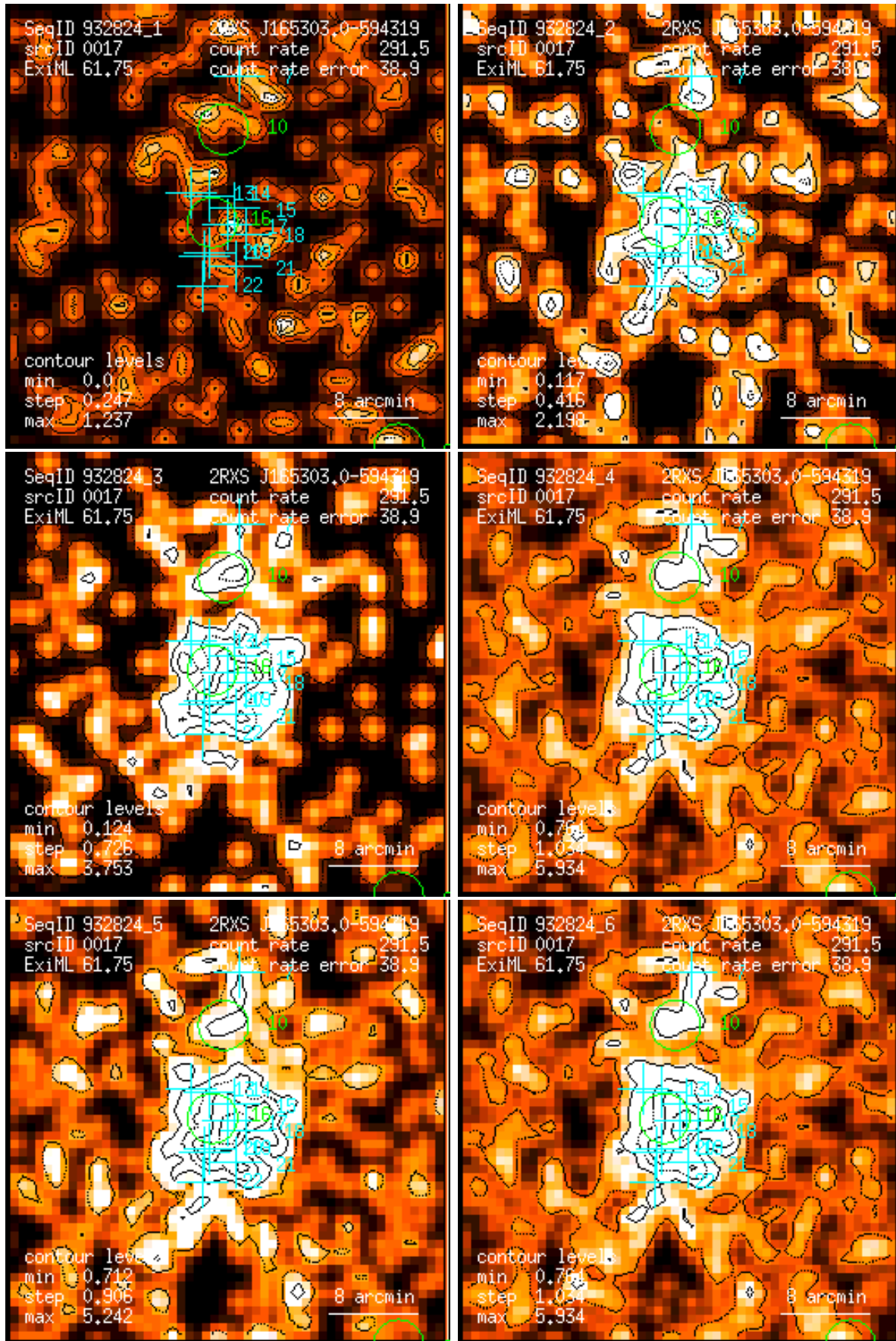
Figure 17: RASS 932824: detection 0017: band rate images, Gaussian filter: (1) PSPC channels 11 – 41, (2) 52 – 90, (3) 91 – 201, (4) 11 – 235, (5) 52 – 201, (6) 11 – 201. Broad band rates in counts/ks. Band rate contour levels in counts/ks/arcmin 2 .
