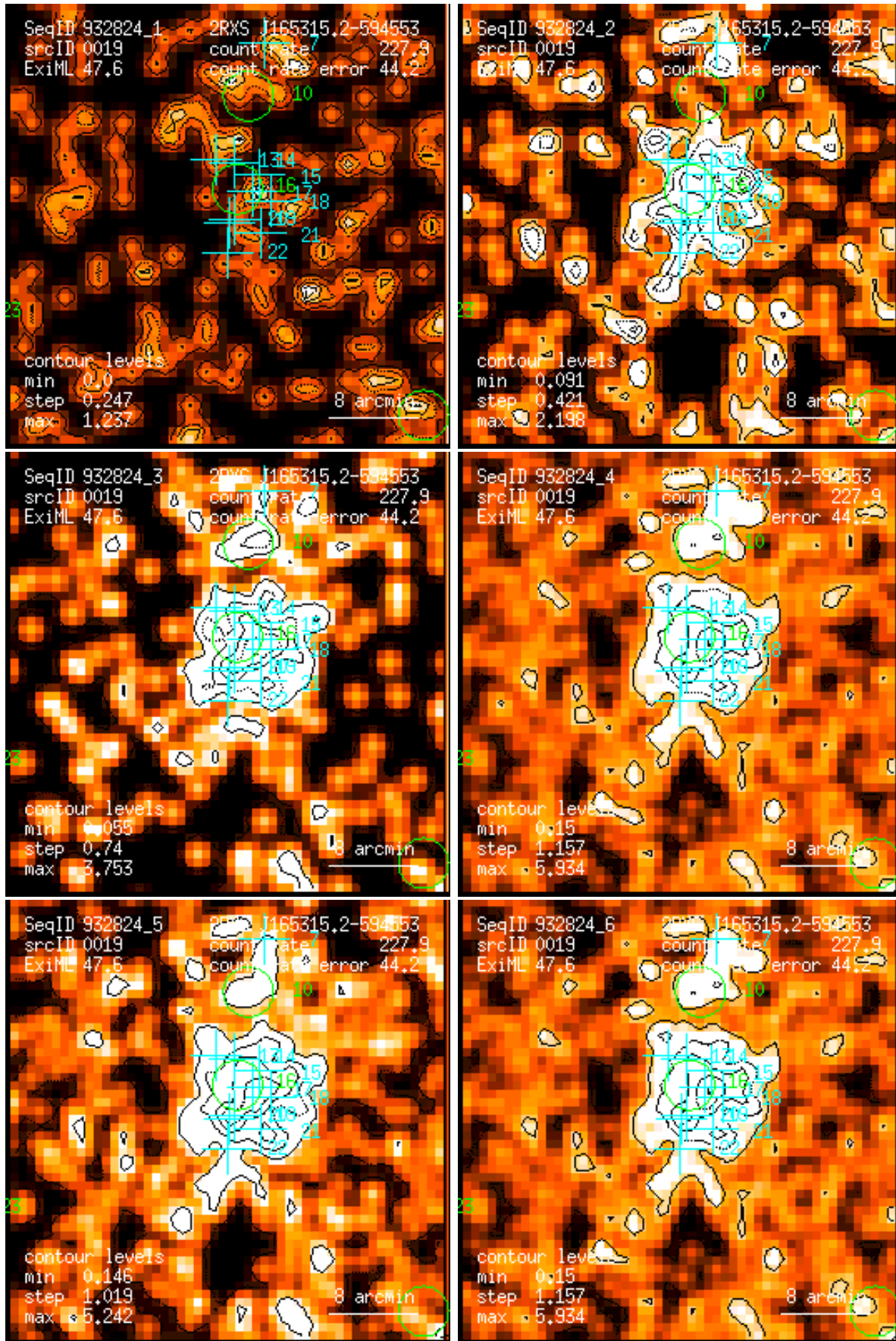
Figure 19: RASS 932824: detection 0019: band rate images, Gaussian filter: (1) PSPC channels 11 – 41, (2) 52 – 90, (3) 91 – 201, (4) 11 – 235, (5) 52 – 201, (6) 11 – 201. Broad band rates in counts/ks. Band rate contour levels in counts/ks/arcmin 2 .
