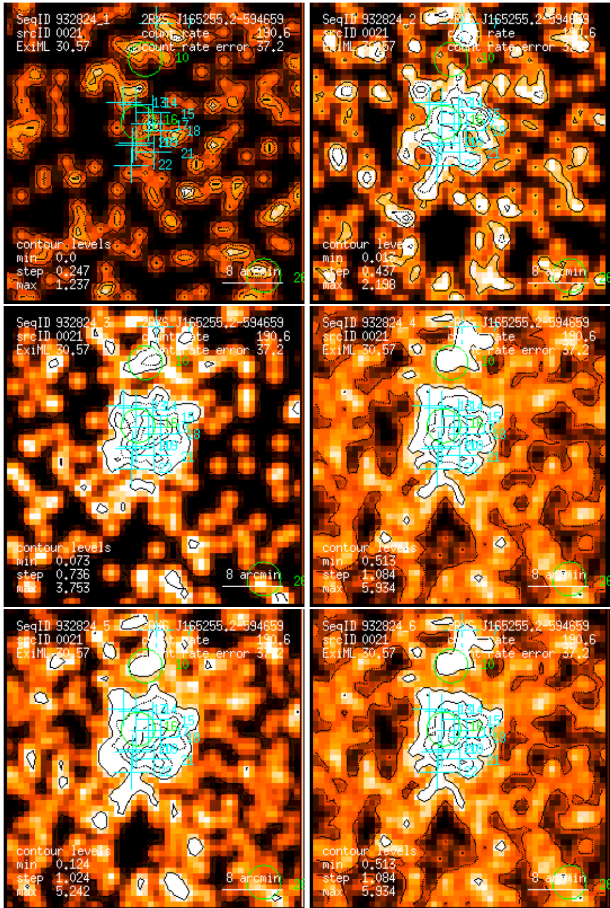
Figure 21: RASS 932824: detection 0021: band rate images, Gaussian filter: (1) PSPC channels 11 – 41, (2) 52 – 90, (3) 91 – 201, (4) 11 – 235, (5) 52 – 201, (6) 11 – 201. Broad band rates in counts/ks. Band rate contour levels in counts/ks/arcmin 2 .
