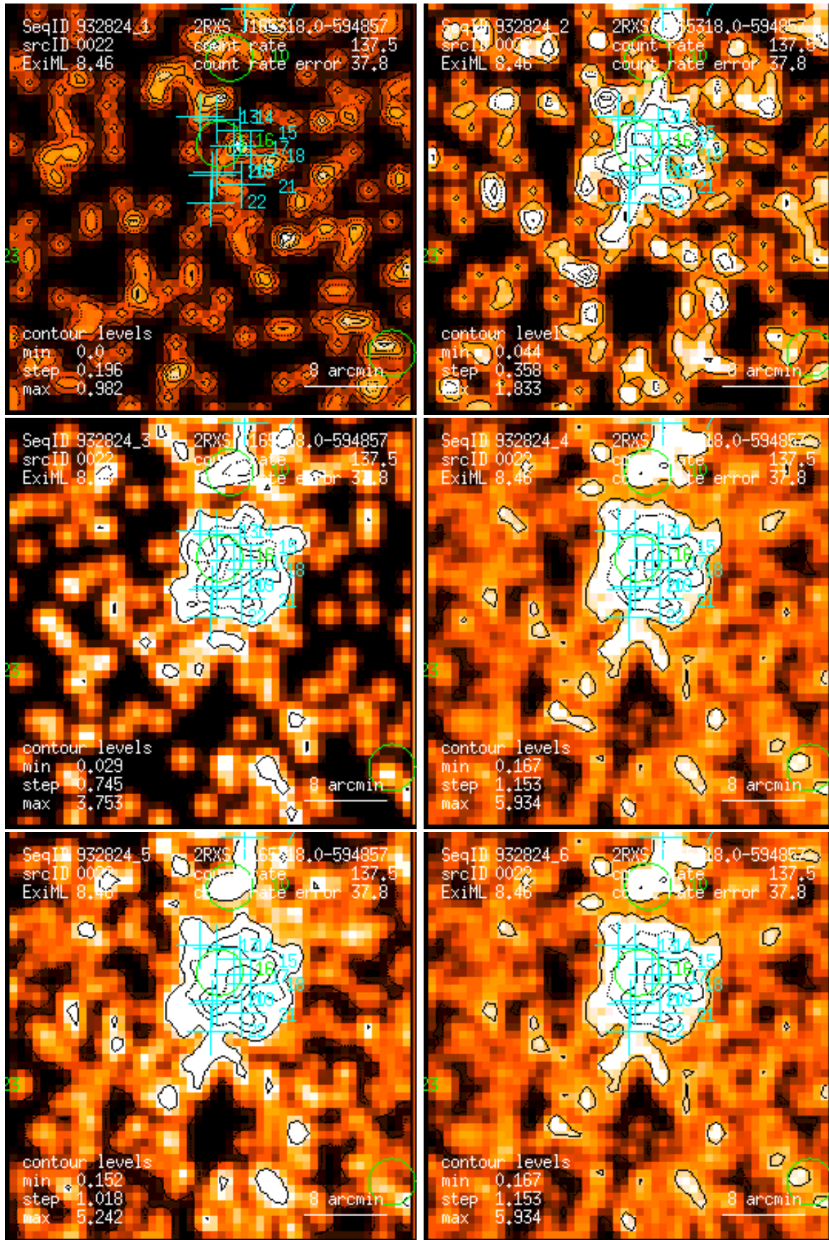
Figure 22: RASS 932824: detection 0022: band rate images, Gaussian filter: (1) PSPC channels 11 – 41, (2) 52 – 90, (3) 91 – 201, (4) 11 – 235, (5) 52 – 201, (6) 11 – 201. Broad band rates in counts/ks. Band rate contour levels in counts/ks/arcmin 2 .
