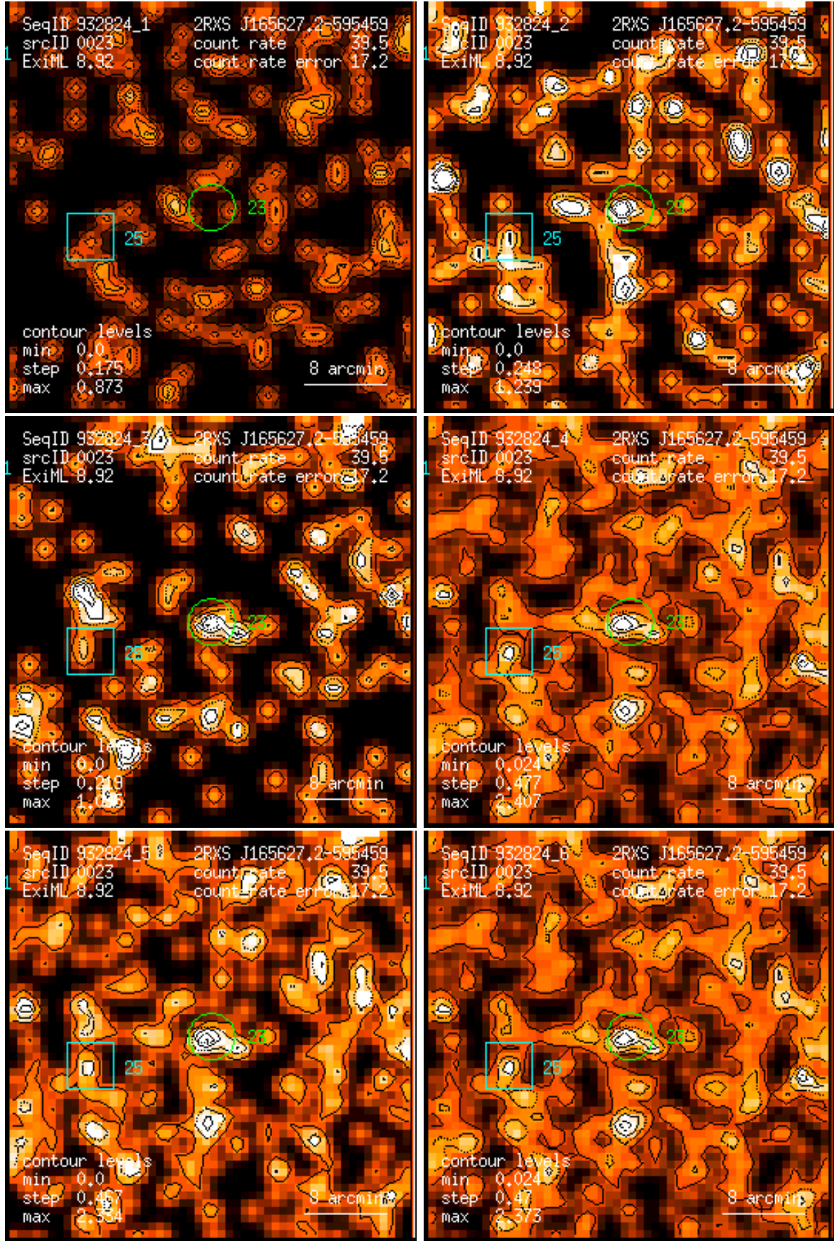
Figure 23: RASS 932824: detection 0023: band rate images, Gaussian filter: (1) PSPC channels 11 – 41, (2) 52 – 90, (3) 91 – 201, (4) 11 – 235, (5) 52 – 201, (6) 11 – 201. Broad band rates in counts/ks. Band rate contour levels in counts/ks/arcmin 2 .
