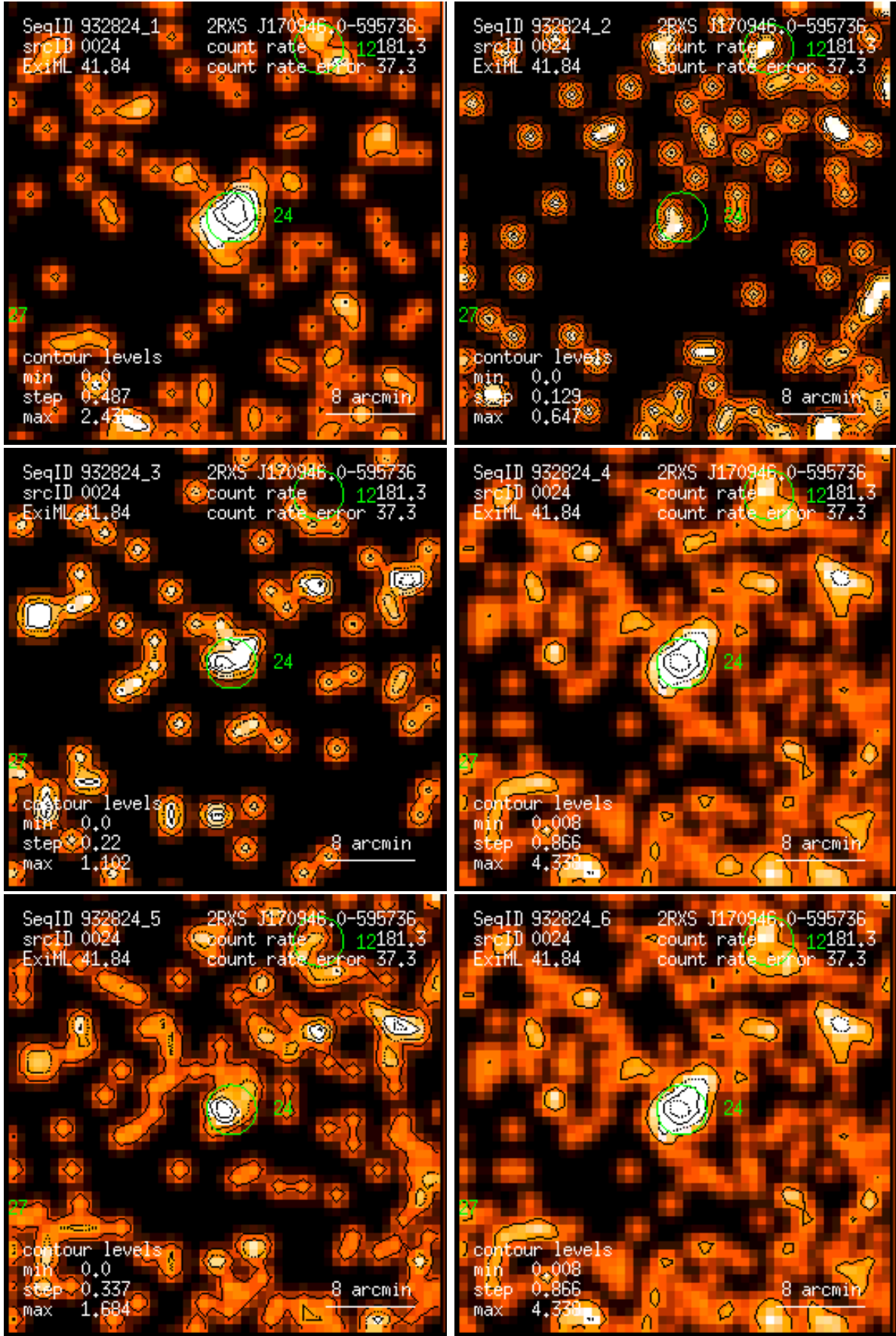
Figure 24: RASS 932824: detection 0024: band rate images, Gaussian filter: (1) PSPC channels 11 – 41, (2) 52 – 90, (3) 91 – 201, (4) 11 – 235, (5) 52 – 201, (6) 11 – 201. Broad band rates in counts/ks. Band rate contour levels in counts/ks/arcmin 2 .
