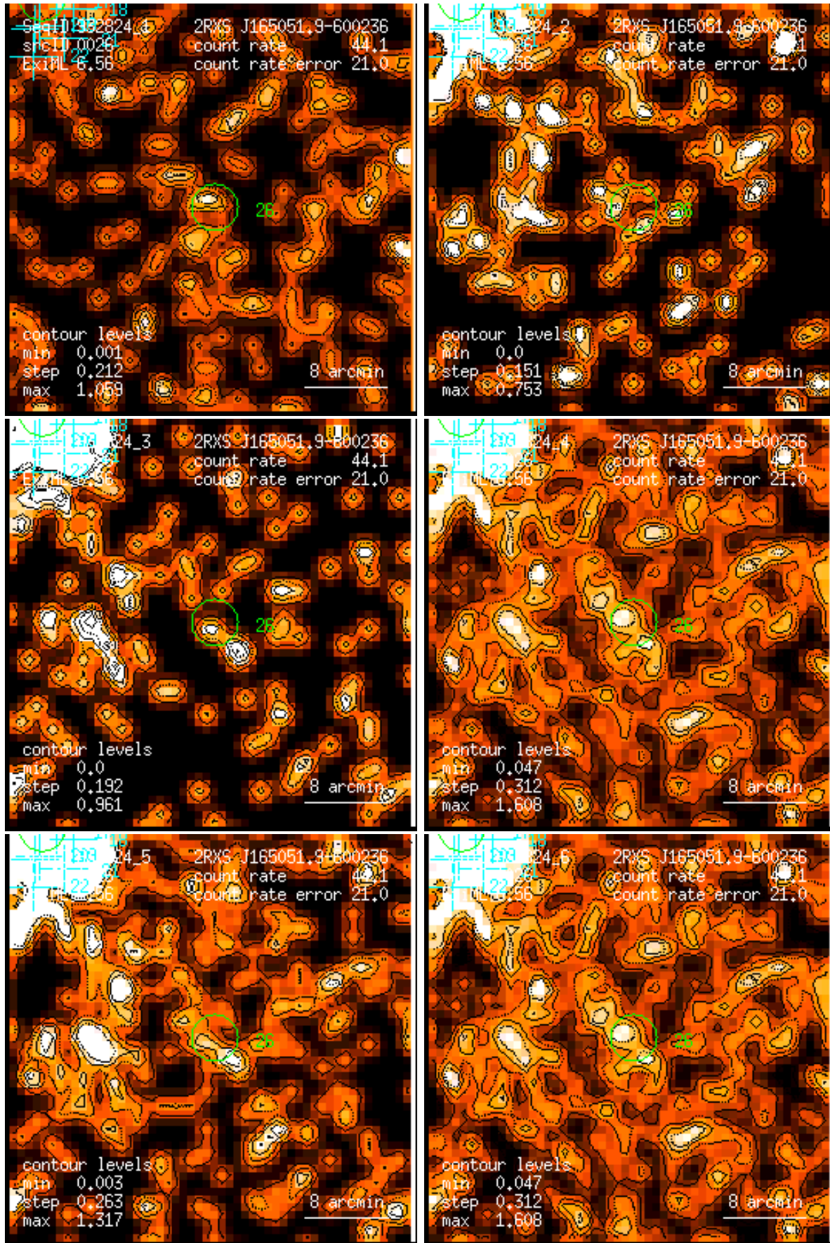
Figure 26: RASS 932824: detection 0026: band rate images, Gaussian filter: (1) PSPC channels 11 – 41, (2) 52 – 90, (3) 91 – 201, (4) 11 – 235, (5) 52 – 201, (6) 11 – 201. Broad band rates in counts/ks. Band rate contour levels in counts/ks/arcmin 2 .
