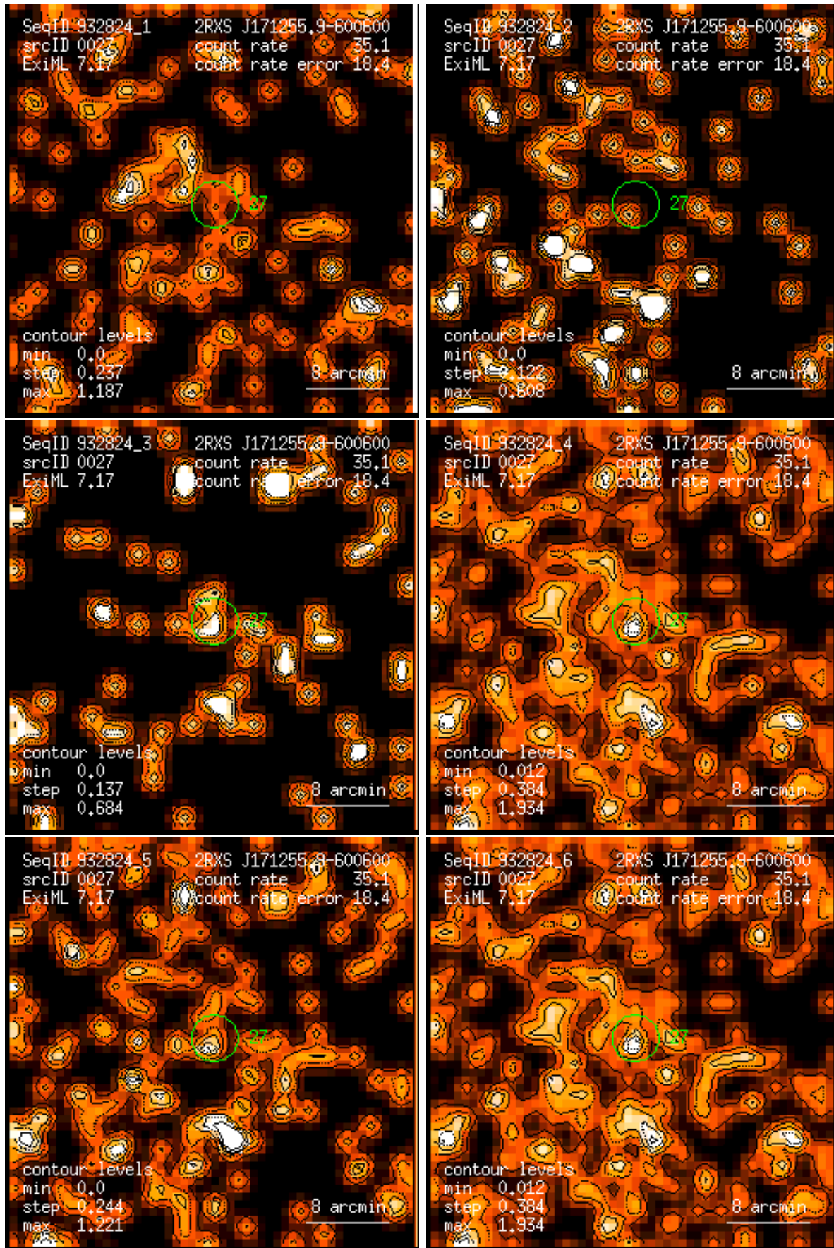
Figure 27: RASS 932824: detection 0027: band rate images, Gaussian filter: (1) PSPC channels 11 – 41, (2) 52 – 90, (3) 91 – 201, (4) 11 – 235, (5) 52 – 201, (6) 11 – 201. Broad band rates in counts/ks. Band rate contour levels in counts/ks/arcmin 2 .
