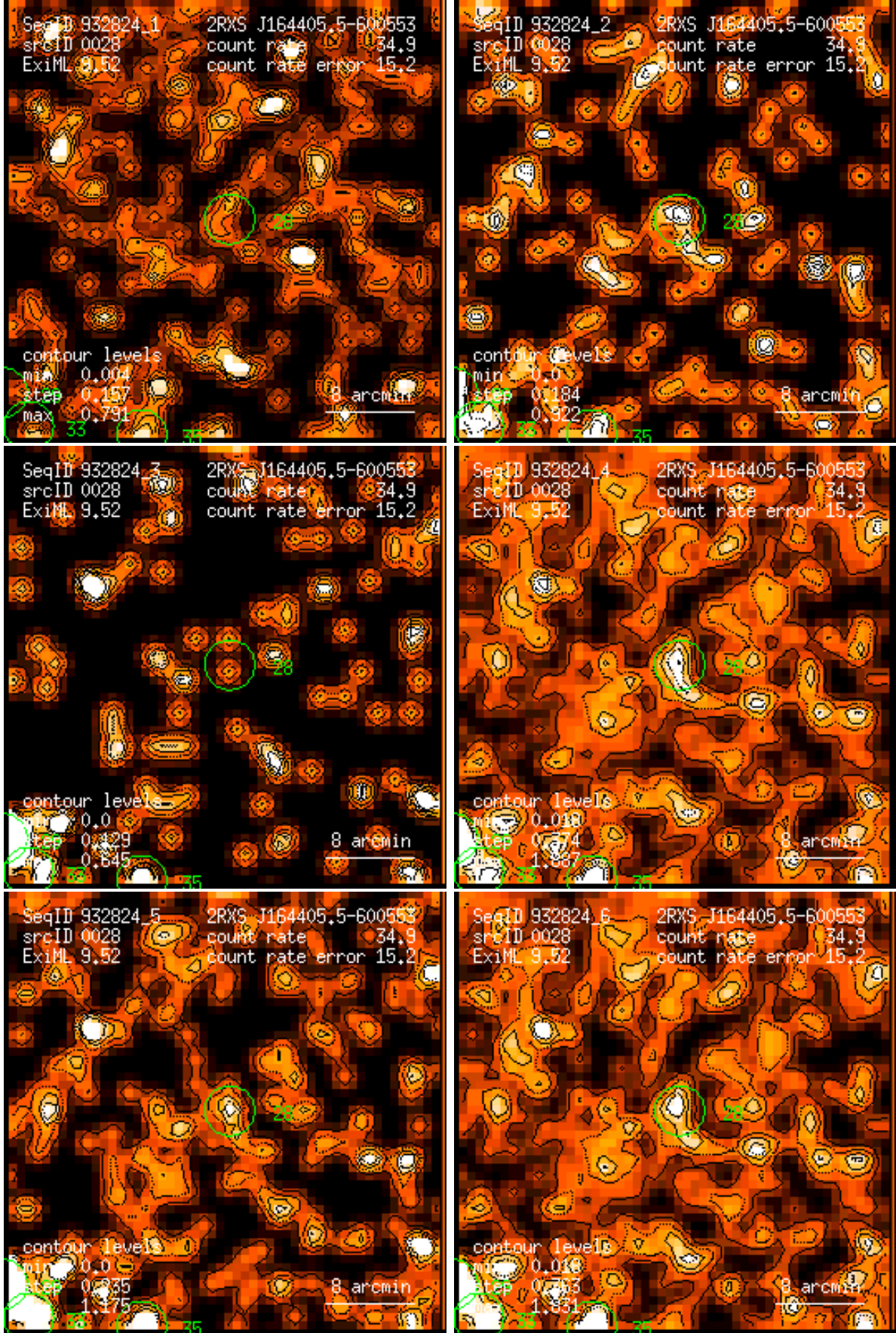
Figure 28: RASS 932824: detection 0028: band rate images, Gaussian filter: (1) PSPC channels 11 – 41, (2) 52 – 90, (3) 91 – 201, (4) 11 – 235, (5) 52 – 201, (6) 11 – 201. Broad band rates in counts/ks. Band rate contour levels in counts/ks/arcmin 2 .
