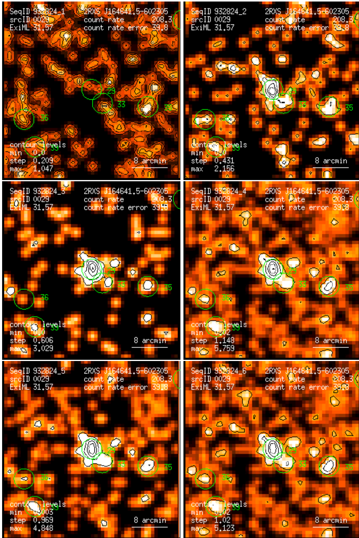
Figure 29: RASS 932824: detection 0029: band rate images, Gaussian filter: (1) PSPC channels 11 – 41, (2) 52 – 90, (3) 91 – 201, (4) 11 – 235, (5) 52 – 201, (6) 11 – 201. Broad band rates in counts/ks. Band rate contour levels in counts/ks/arcmin 2 .
