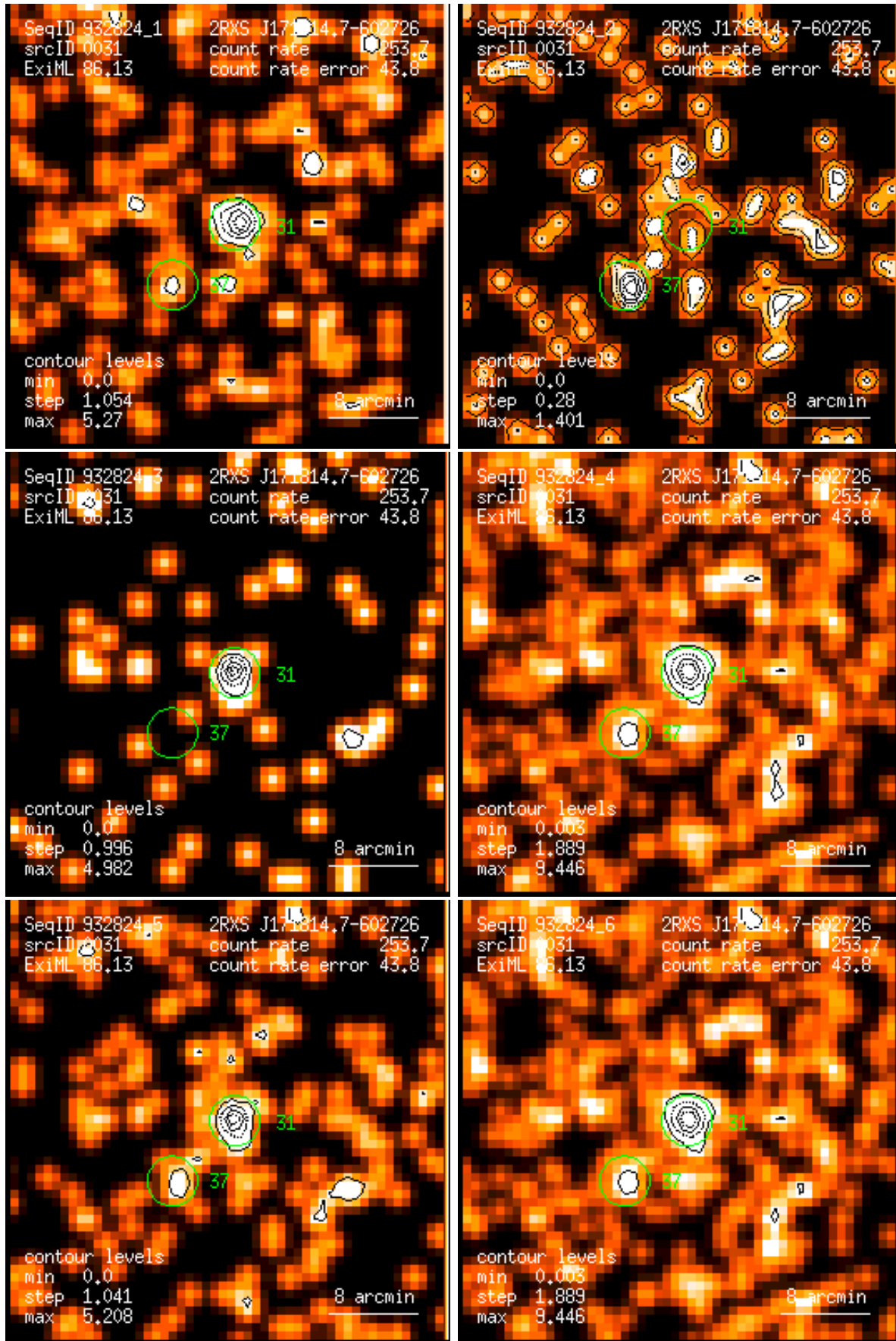
Figure 31: RASS 932824: detection 0031: band rate images, Gaussian filter: (1) PSPC channels 11 – 41, (2) 52 – 90, (3) 91 – 201, (4) 11 – 235, (5) 52 – 201, (6) 11 – 201. Broad band rates in counts/ks. Band rate contour levels in counts/ks/arcmin 2 .
