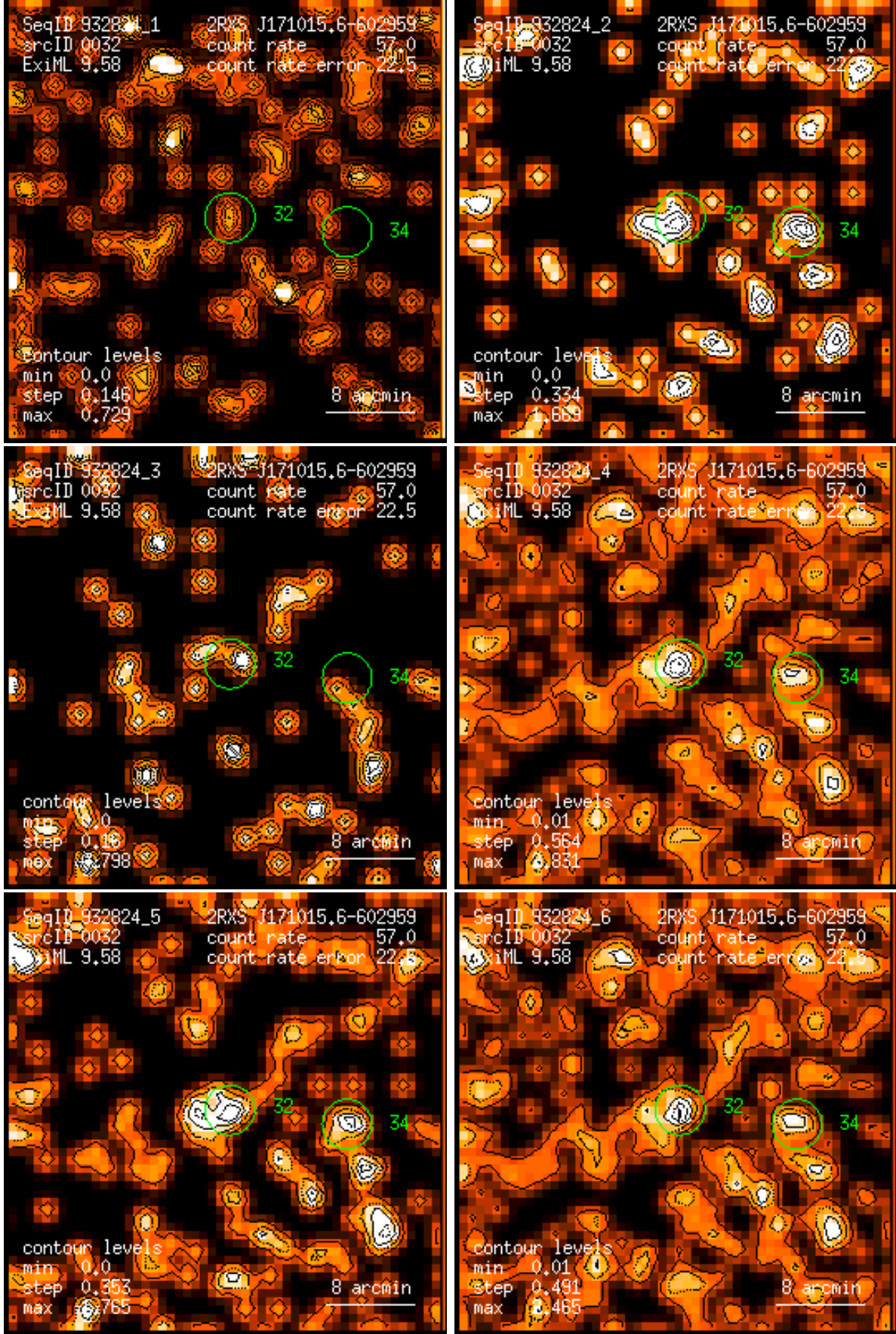
Figure 32: RASS 932824: detection 0032: band rate images, Gaussian filter: (1) PSPC channels 11 – 41, (2) 52 – 90, (3) 91 – 201, (4) 11 – 235, (5) 52 – 201, (6) 11 – 201. Broad band rates in counts/ks. Band rate contour levels in counts/ks/arcmin 2 .
