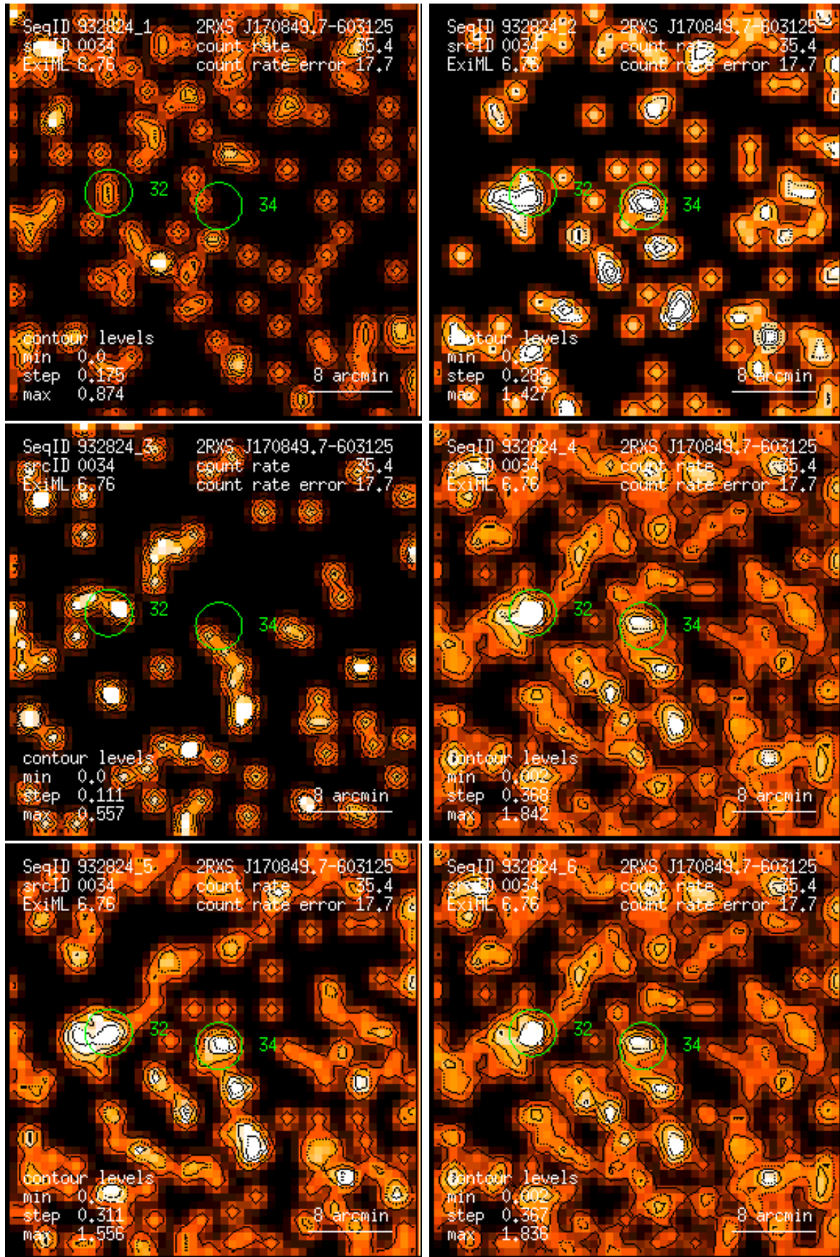
Figure 34: RASS 932824: detection 0034: band rate images, Gaussian filter: (1) PSPC channels 11 – 41, (2) 52 – 90, (3) 91 – 201, (4) 11 – 235, (5) 52 – 201, (6) 11 – 201. Broad band rates in counts/ks. Band rate contour levels in counts/ks/arcmin 2 .
