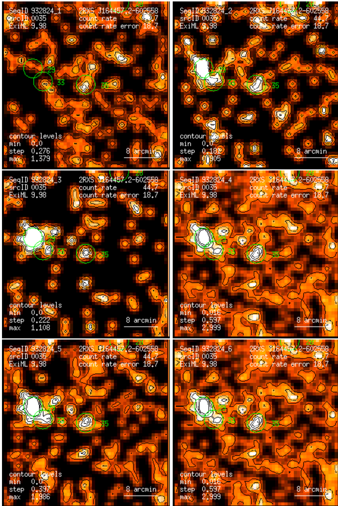
Figure 35: RASS 932824: detection 0035: band rate images, Gaussian filter: (1) PSPC channels 11 – 41, (2) 52 – 90, (3) 91 – 201, (4) 11 – 235, (5) 52 – 201, (6) 11 – 201. Broad band rates in counts/ks. Band rate contour levels in counts/ks/arcmin 2 .
