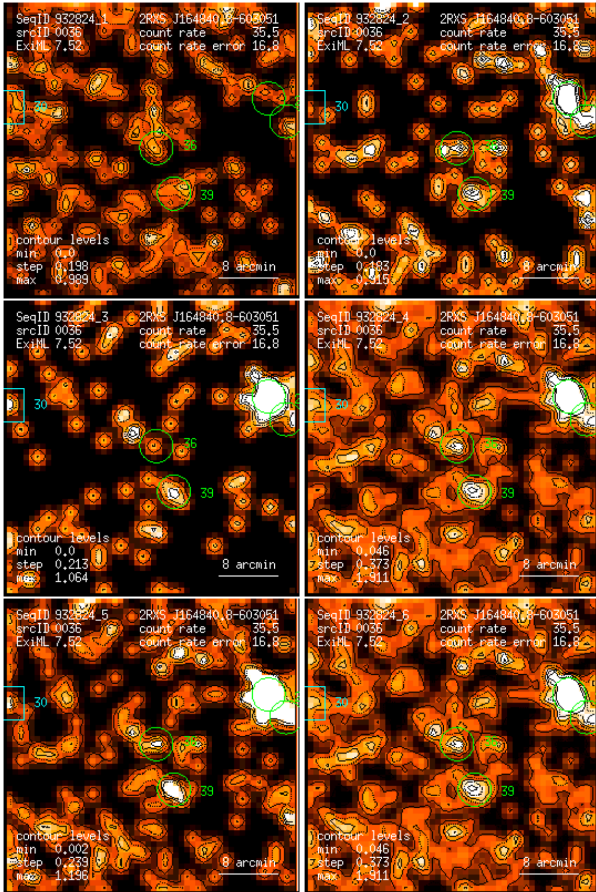
Figure 36: RASS 932824: detection 0036: band rate images, Gaussian filter: (1) PSPC channels 11 – 41, (2) 52 – 90, (3) 91 – 201, (4) 11 – 235, (5) 52 – 201, (6) 11 – 201. Broad band rates in counts/ks. Band rate contour levels in counts/ks/arcmin 2 .
