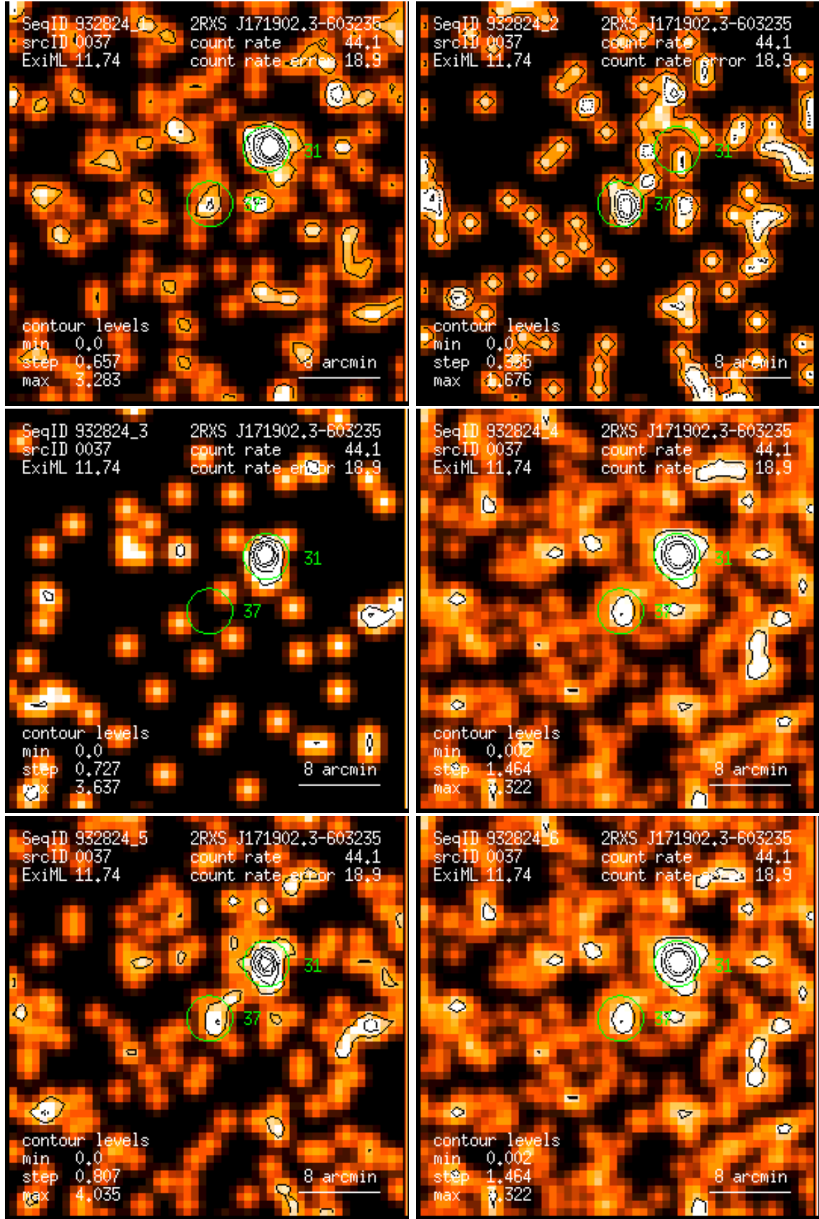
Figure 37: RASS 932824: detection 0037: band rate images, Gaussian filter: (1) PSPC channels 11 – 41, (2) 52 – 90, (3) 91 – 201, (4) 11 – 235, (5) 52 – 201, (6) 11 – 201. Broad band rates in counts/ks. Band rate contour levels in counts/ks/arcmin 2 .
