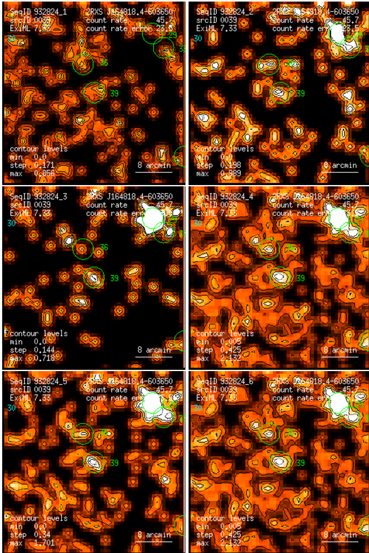
Figure 39: RASS 932824: detection 0039: band rate images, Gaussian filter: (1) PSPC channels 11 – 41, (2) 52 – 90, (3) 91 – 201, (4) 11 – 235, (5) 52 – 201, (6) 11 – 201. Broad band rates in counts/ks. Band rate contour levels in counts/ks/arcmin 2 .
