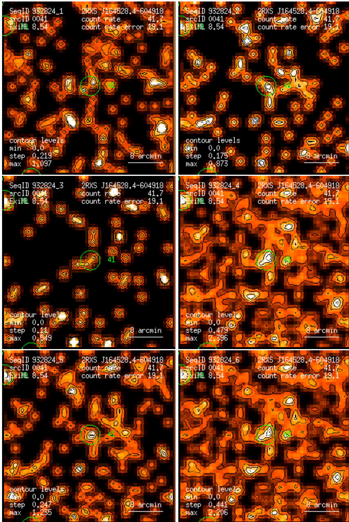
Figure 41: RASS 932824: detection 0041: band rate images, Gaussian filter: (1) PSPC channels 11 – 41, (2) 52 – 90, (3) 91 – 201, (4) 11 – 235, (5) 52 – 201, (6) 11 – 201. Broad band rates in counts/ks. Band rate contour levels in counts/ks/arcmin 2 .
