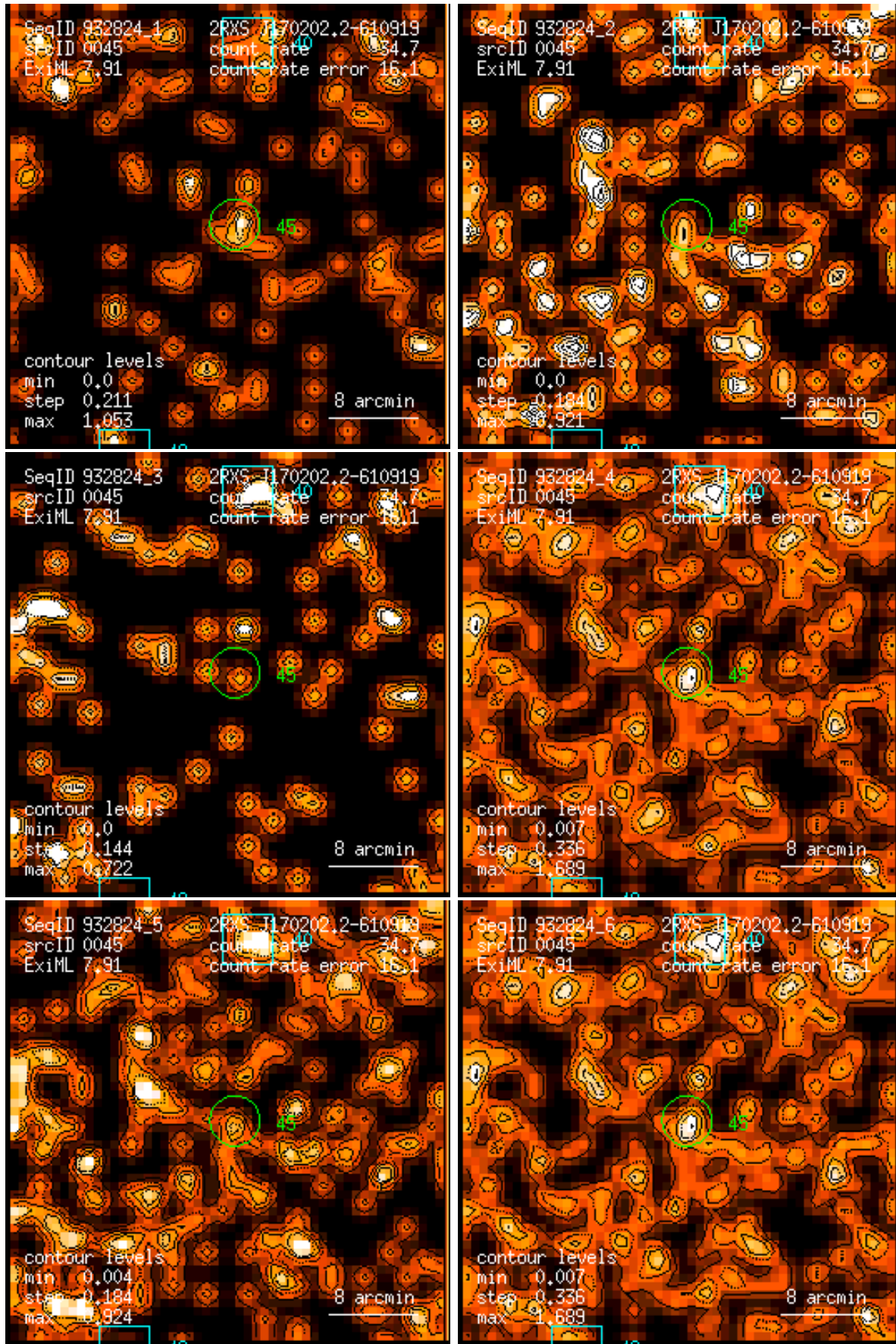
Figure 45: RASS 932824: detection 0045: band rate images, Gaussian filter: (1) PSPC channels 11 – 41, (2) 52 – 90, (3) 91 – 201, (4) 11 – 235, (5) 52 – 201, (6) 11 – 201. Broad band rates in counts/ks. Band rate contour levels in counts/ks/arcmin 2 .
