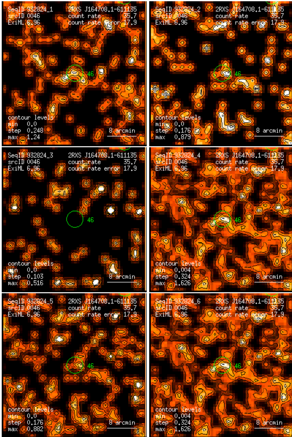
Figure 46: RASS 932824: detection 0046: band rate images, Gaussian filter: (1) PSPC channels 11 – 41, (2) 52 – 90, (3) 91 – 201, (4) 11 – 235, (5) 52 – 201, (6) 11 – 201. Broad band rates in counts/ks. Band rate contour levels in counts/ks/arcmin 2 .
