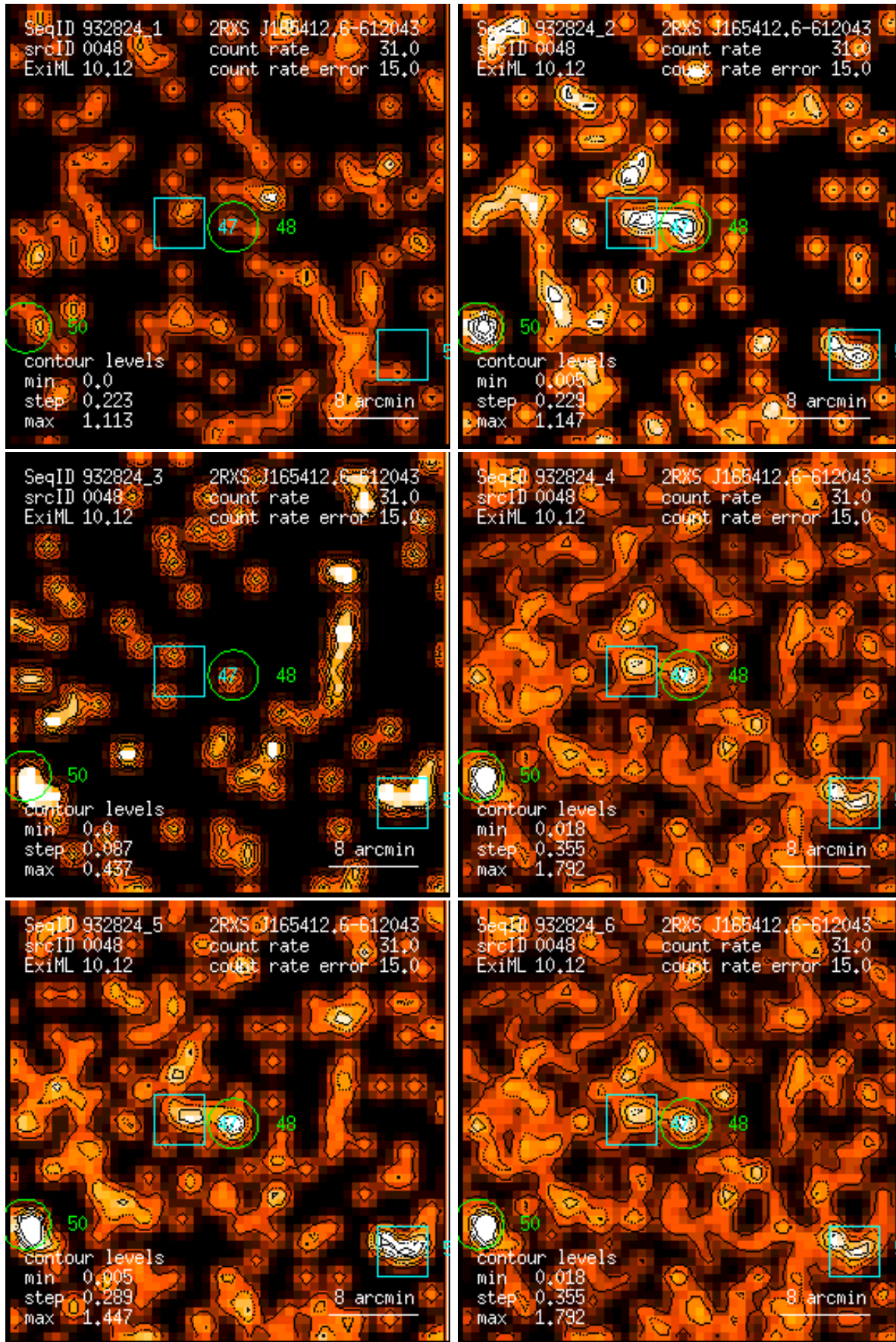
Figure 48: RASS 932824: detection 0048: band rate images, Gaussian filter: (1) PSPC channels 11 – 41, (2) 52 – 90, (3) 91 – 201, (4) 11 – 235, (5) 52 – 201, (6) 11 – 201. Broad band rates in counts/ks. Band rate contour levels in counts/ks/arcmin 2 .
