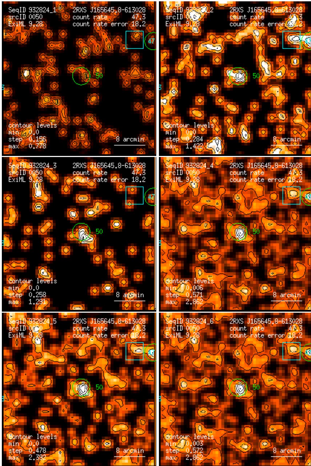
Figure 50: RASS 932824: detection 0050: band rate images, Gaussian filter: (1) PSPC channels 11 – 41, (2) 52 – 90, (3) 91 – 201, (4) 11 – 235, (5) 52 – 201, (6) 11 – 201. Broad band rates in counts/ks. Band rate contour levels in counts/ks/arcmin 2 .
