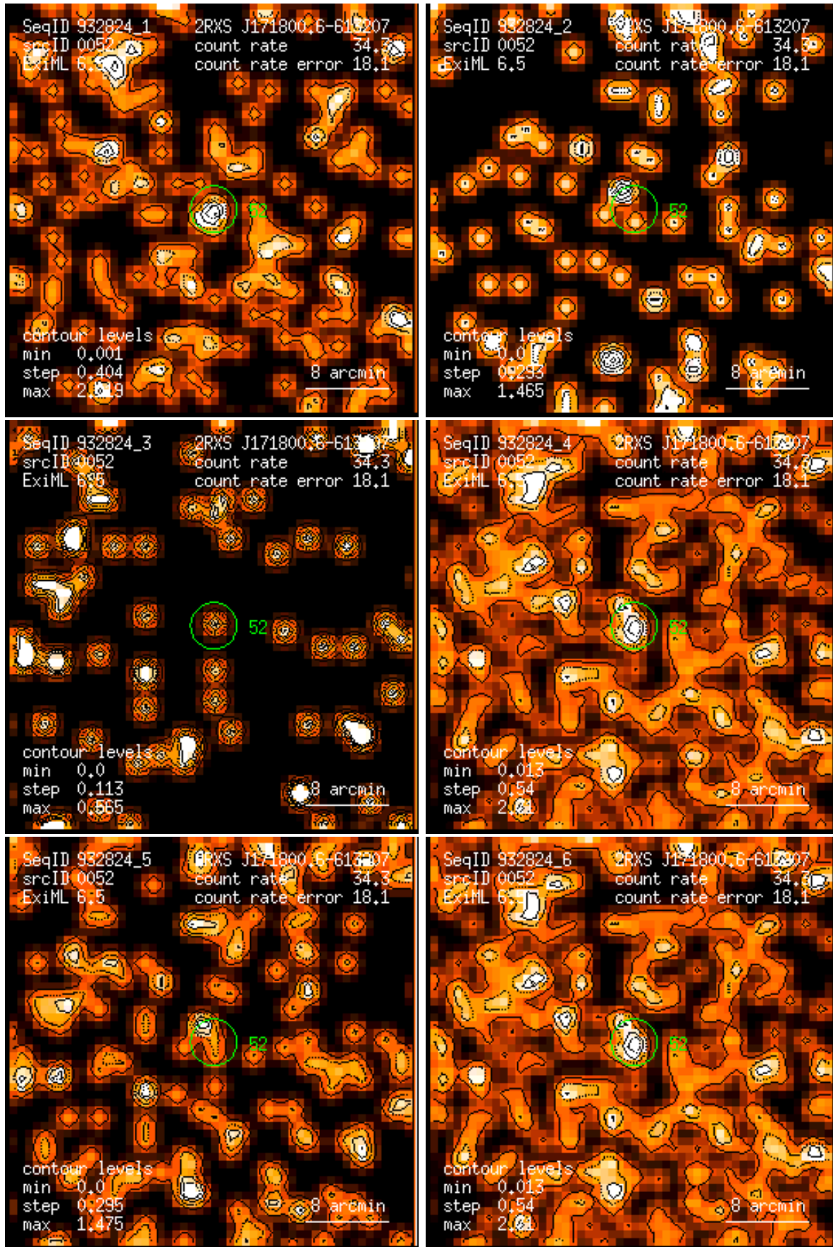
Figure 52: RASS 932824: detection 0052: band rate images, Gaussian filter: (1) PSPC channels 11 – 41, (2) 52 – 90, (3) 91 – 201, (4) 11 – 235, (5) 52 – 201, (6) 11 – 201. Broad band rates in counts/ks. Band rate contour levels in counts/ks/arcmin 2 .
