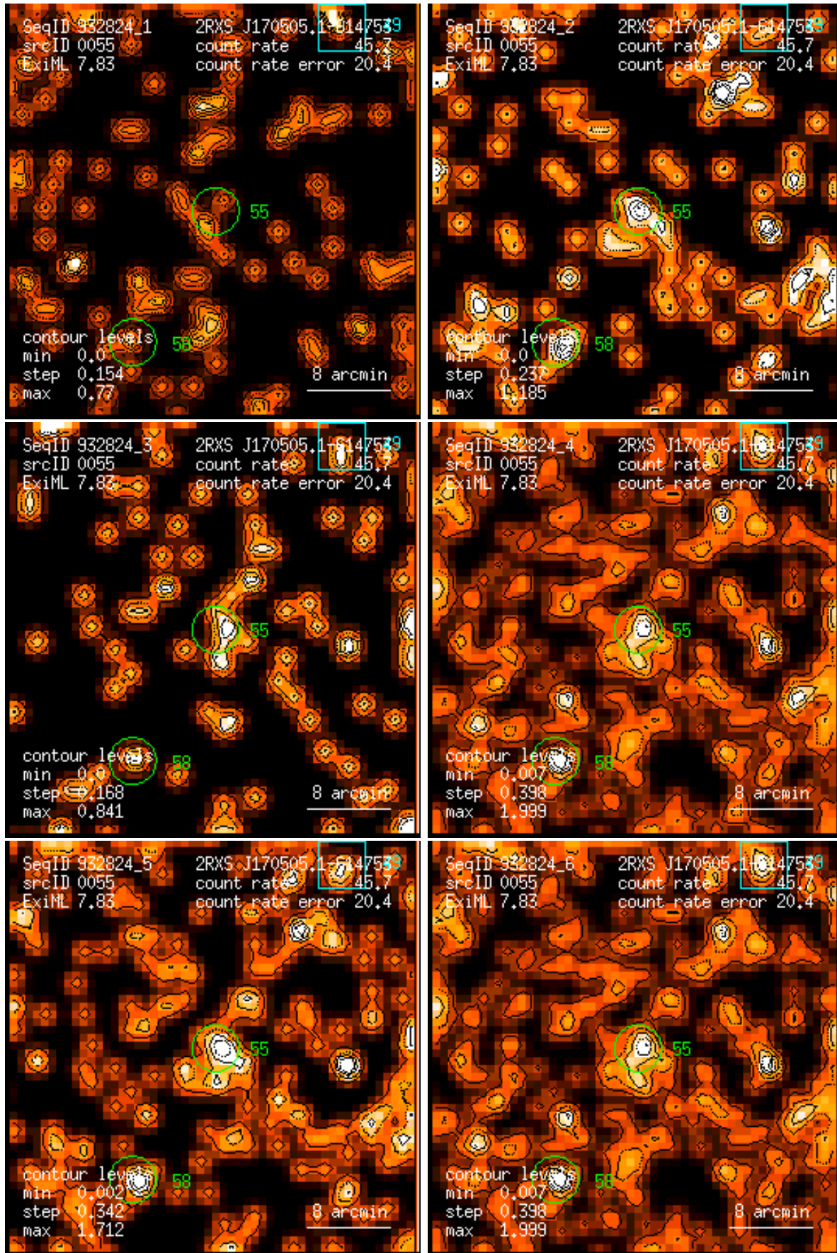
Figure 55: RASS 932824: detection 0055: band rate images, Gaussian filter: (1) PSPC channels 11 – 41, (2) 52 – 90, (3) 91 – 201, (4) 11 – 235, (5) 52 – 201, (6) 11 – 201. Broad band rates in counts/ks. Band rate contour levels in counts/ks/arcmin 2 .
