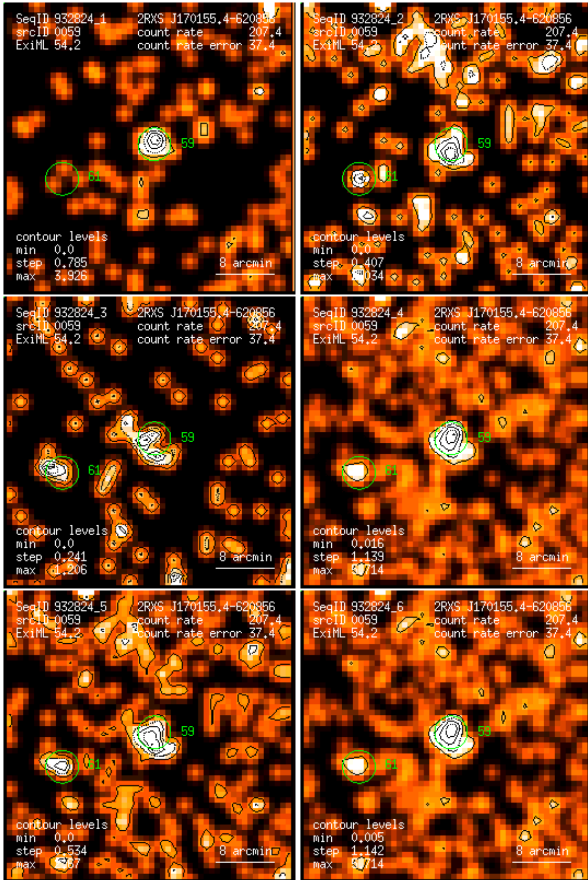
Figure 59: RASS 932824: detection 0059: band rate images, Gaussian filter: (1) PSPC channels 11 – 41, (2) 52 – 90, (3) 91 – 201, (4) 11 – 235, (5) 52 – 201, (6) 11 – 201. Broad band rates in counts/ks. Band rate contour levels in counts/ks/arcmin 2 .
