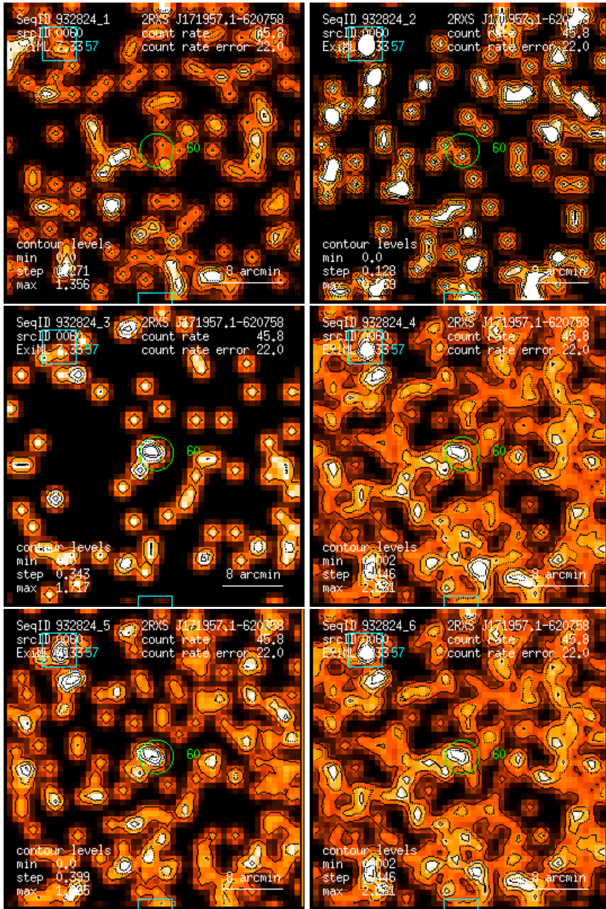
Figure 60: RASS 932824: detection 0060: band rate images, Gaussian filter: (1) PSPC channels 11 – 41, (2) 52 – 90, (3) 91 – 201, (4) 11 – 235, (5) 52 – 201, (6) 11 – 201. Broad band rates in counts/ks. Band rate contour levels in counts/ks/arcmin 2 .
