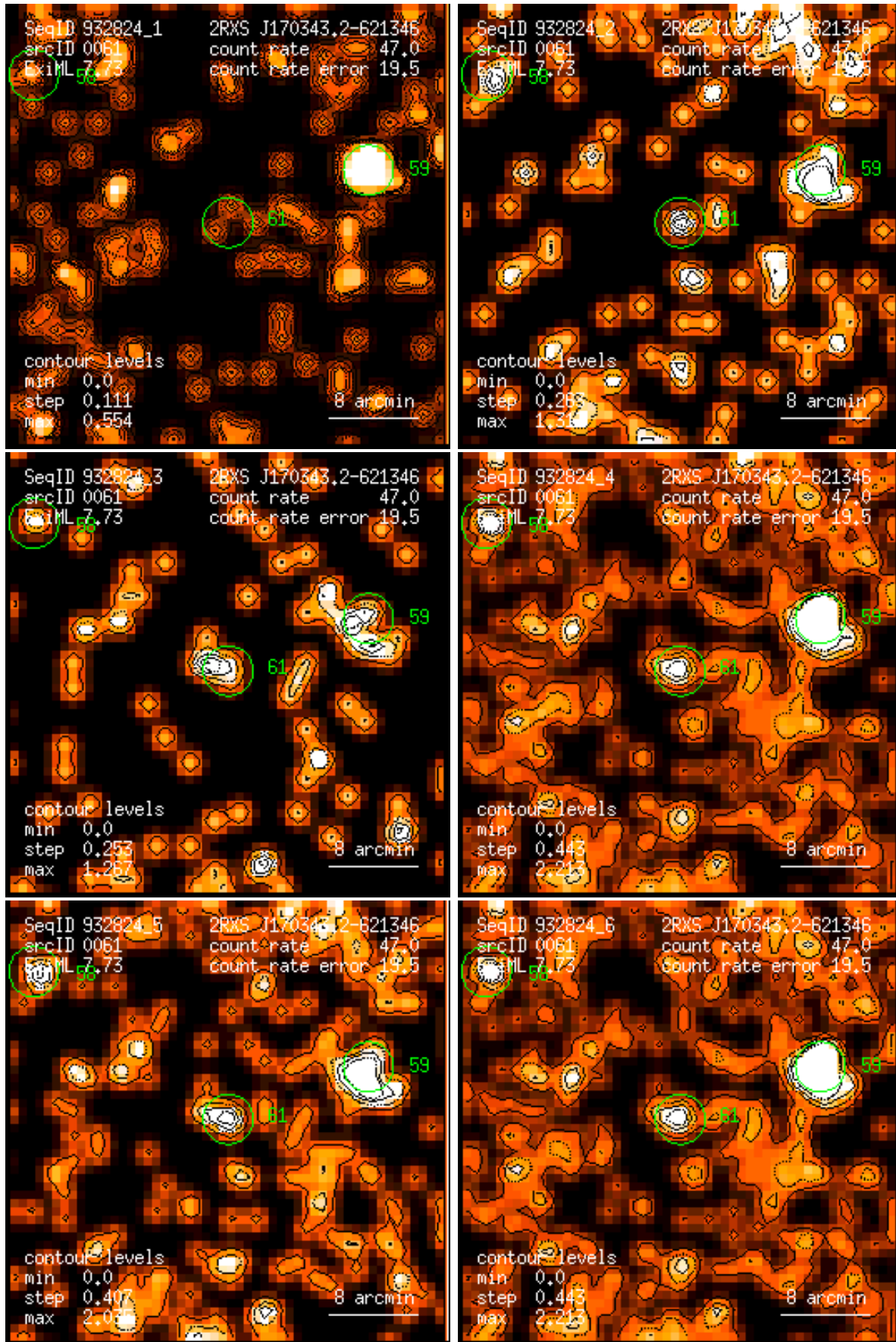
Figure 61: RASS 932824: detection 0061: band rate images, Gaussian filter: (1) PSPC channels 11 – 41, (2) 52 – 90, (3) 91 – 201, (4) 11 – 235, (5) 52 – 201, (6) 11 – 201. Broad band rates in counts/ks. Band rate contour levels in counts/ks/arcmin 2 .
