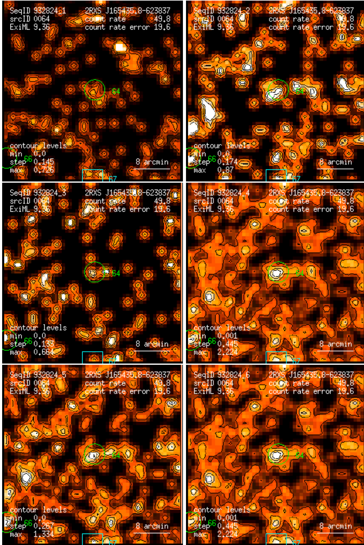
Figure 64: RASS 932824: detection 0064: band rate images, Gaussian filter: (1) PSPC channels 11 – 41, (2) 52 – 90, (3) 91 – 201, (4) 11 – 235, (5) 52 – 201, (6) 11 – 201. Broad band rates in counts/ks. Band rate contour levels in counts/ks/arcmin 2 .
