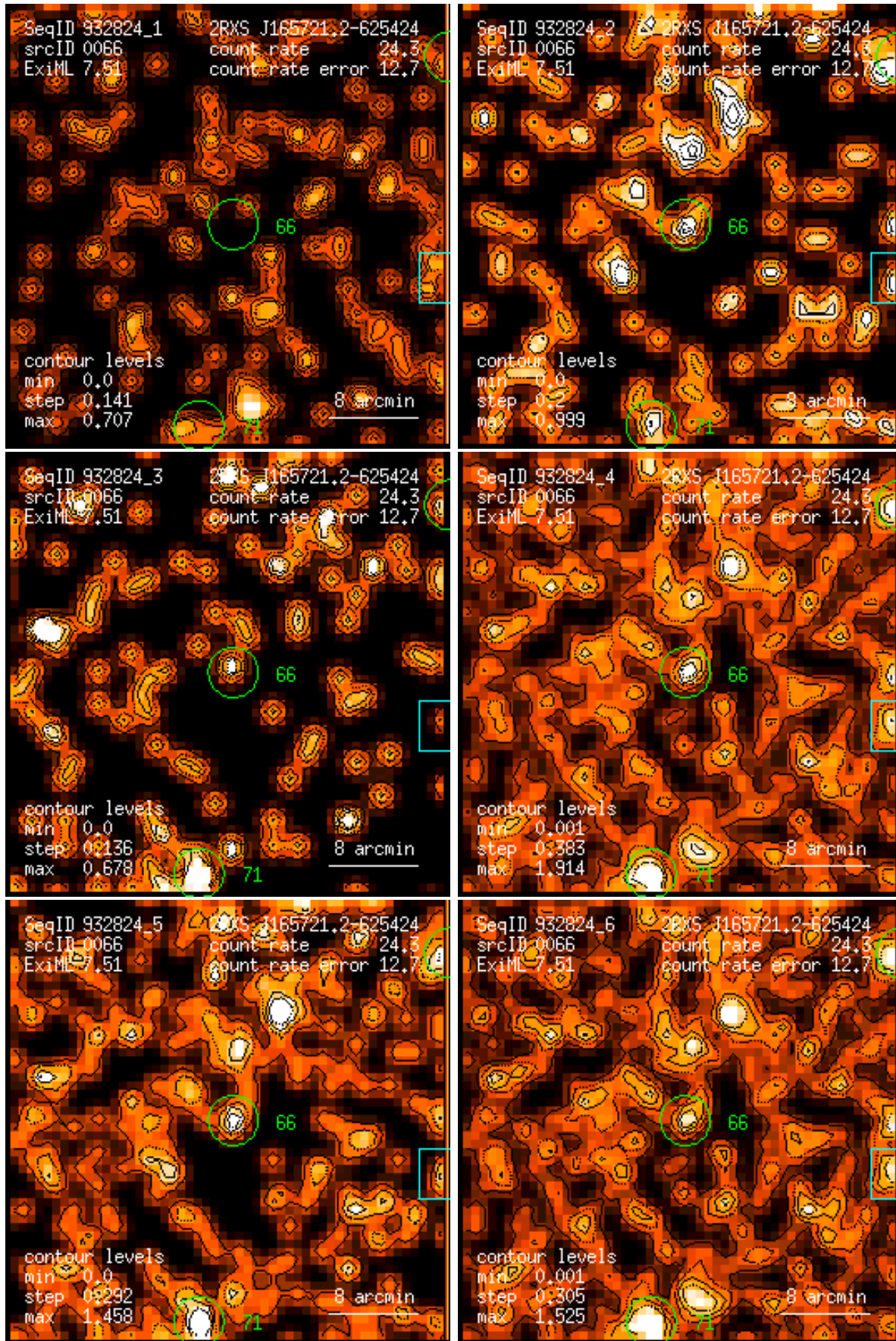
Figure 66: RASS 932824: detection 0066: band rate images, Gaussian filter: (1) PSPC channels 11 – 41, (2) 52 – 90, (3) 91 – 201, (4) 11 – 235, (5) 52 – 201, (6) 11 – 201. Broad band rates in counts/ks. Band rate contour levels in counts/ks/arcmin 2 .
