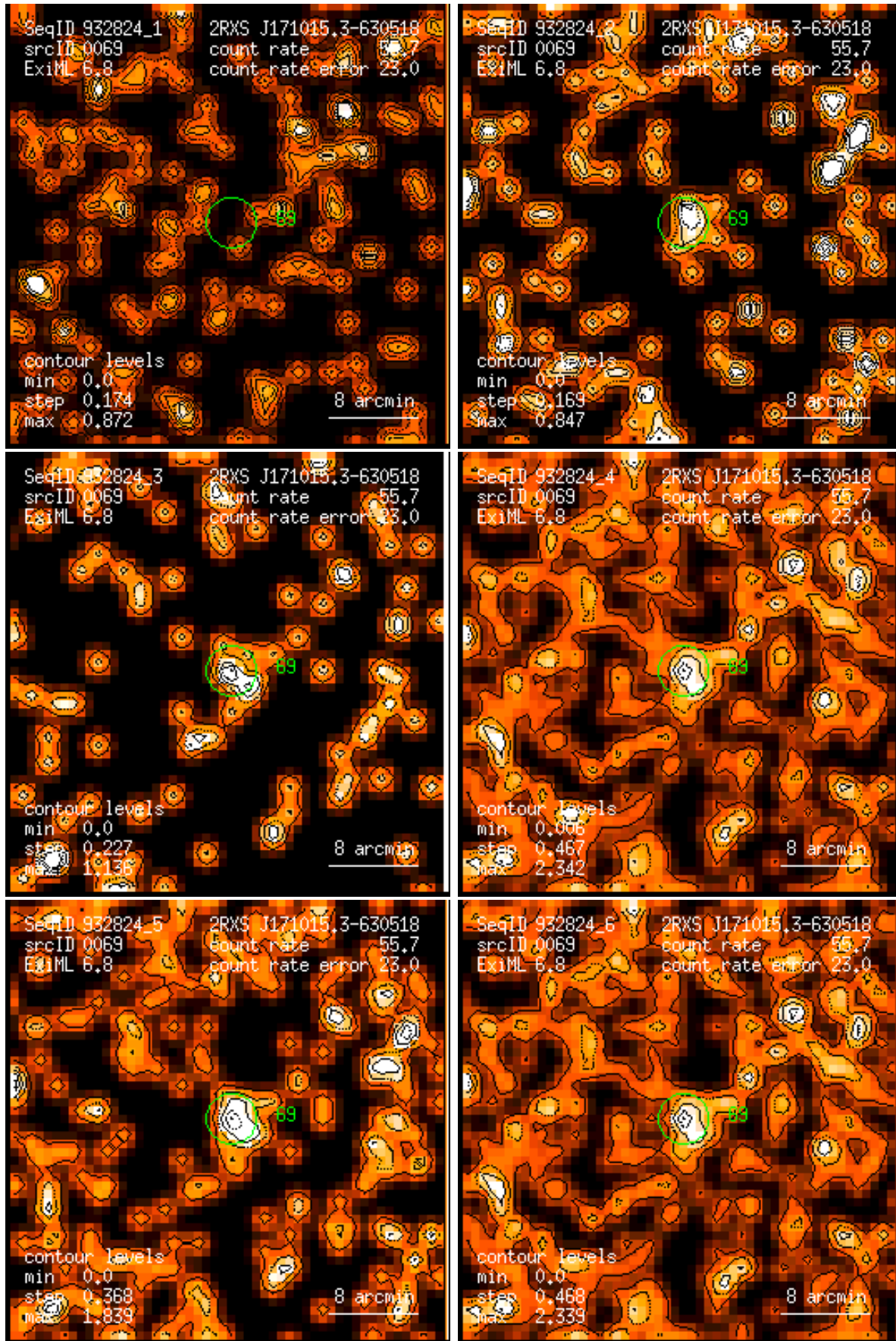
Figure 69: RASS 932824: detection 0069: band rate images, Gaussian filter: (1) PSPC channels 11 – 41, (2) 52 – 90, (3) 91 – 201, (4) 11 – 235, (5) 52 – 201, (6) 11 – 201. Broad band rates in counts/ks. Band rate contour levels in counts/ks/arcmin 2 .
