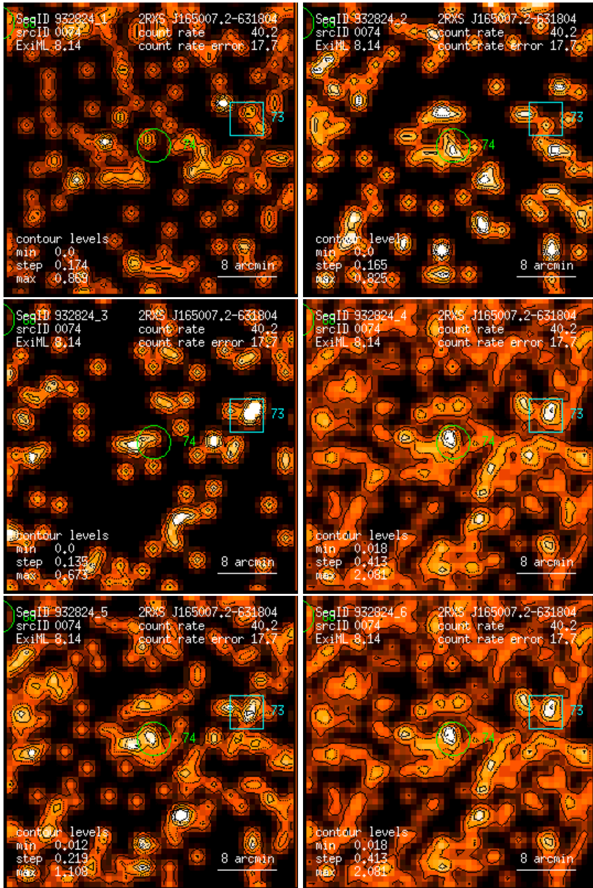
Figure 74: RASS 932824: detection 0074: band rate images, Gaussian filter: (1) PSPC channels 11 – 41, (2) 52 – 90, (3) 91 – 201, (4) 11 – 235, (5) 52 – 201, (6) 11 – 201. Broad band rates in counts/ks. Band rate contour levels in counts/ks/arcmin 2 .
