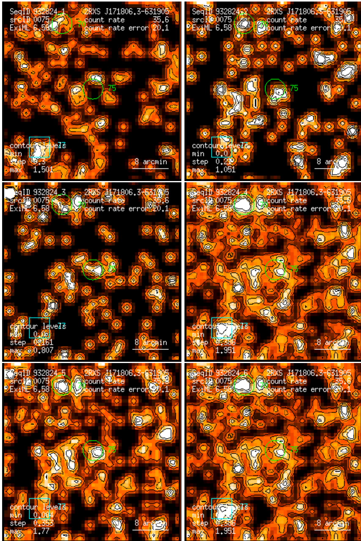
Figure 75: RASS 932824: detection 0075: band rate images, Gaussian filter: (1) PSPC channels 11 – 41, (2) 52 – 90, (3) 91 – 201, (4) 11 – 235, (5) 52 – 201, (6) 11 – 201. Broad band rates in counts/ks. Band rate contour levels in counts/ks/arcmin 2 .
