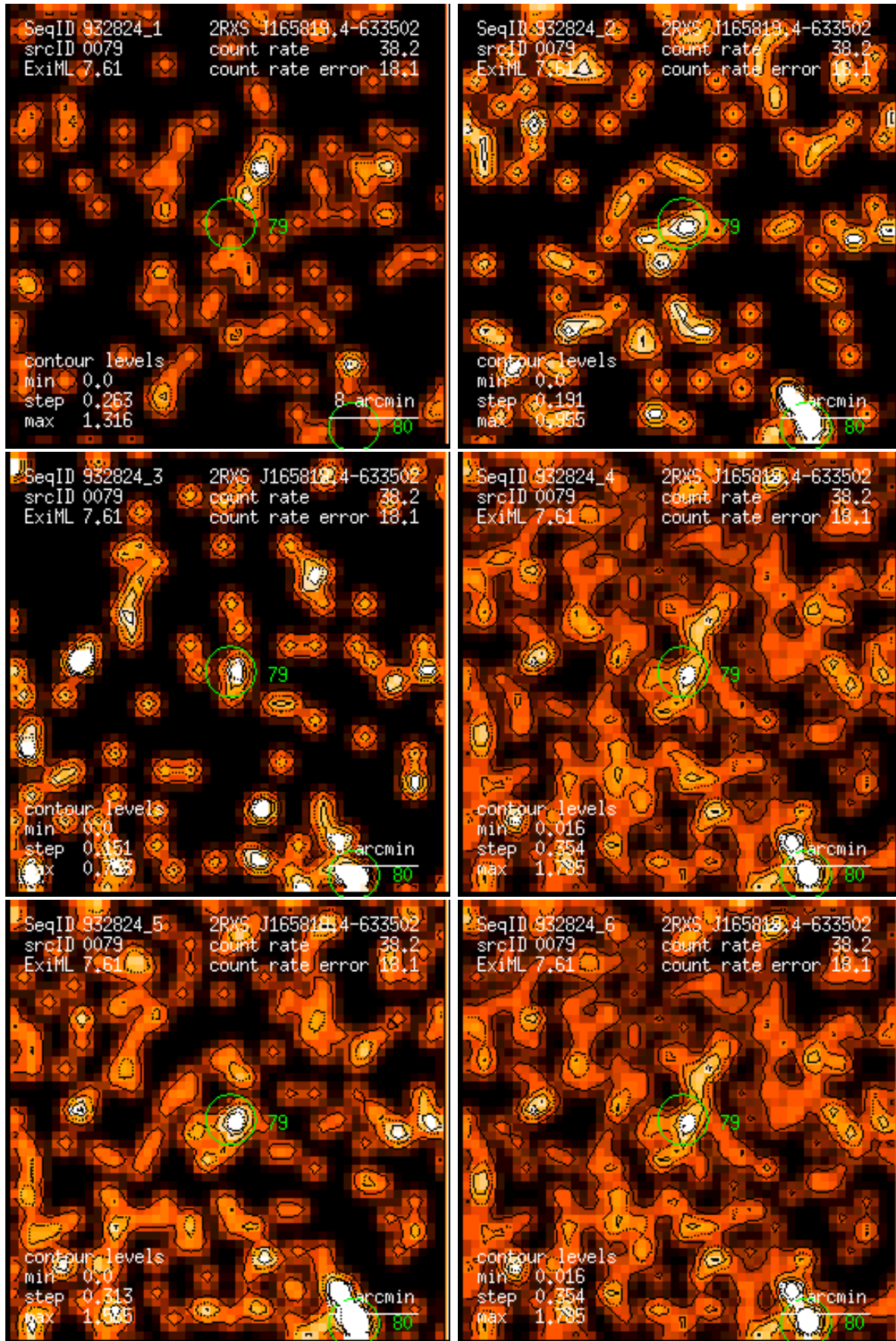
Figure 79: RASS 932824: detection 0079: band rate images, Gaussian filter: (1) PSPC channels 11 – 41, (2) 52 – 90, (3) 91 – 201, (4) 11 – 235, (5) 52 – 201, (6) 11 – 201. Broad band rates in counts/ks. Band rate contour levels in counts/ks/arcmin 2 .
