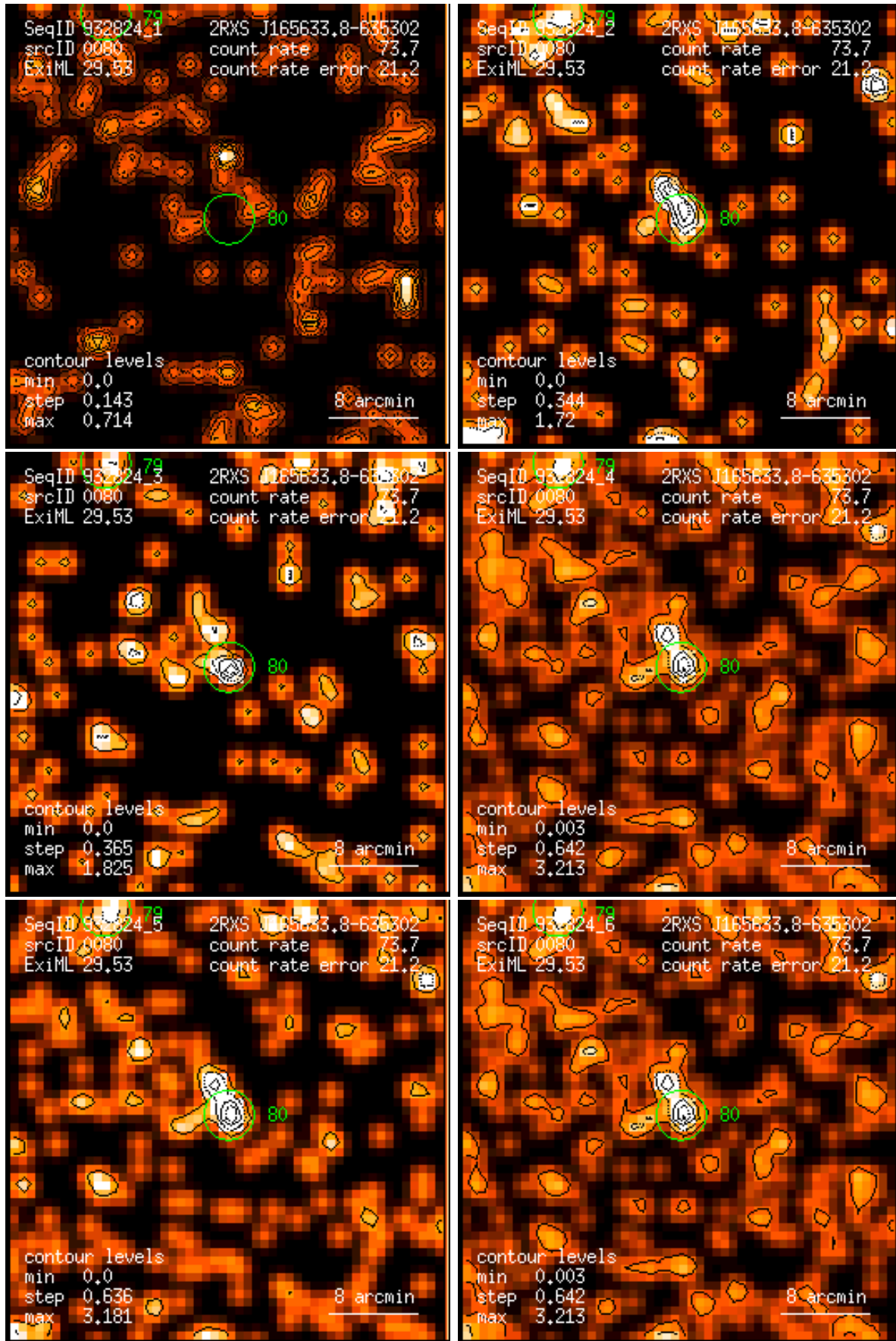
Figure 80: RASS 932824: detection 0080: band rate images, Gaussian filter: (1) PSPC channels 11 – 41, (2) 52 – 90, (3) 91 – 201, (4) 11 – 235, (5) 52 – 201, (6) 11 – 201. Broad band rates in counts/ks. Band rate contour levels in counts/ks/arcmin 2 .
