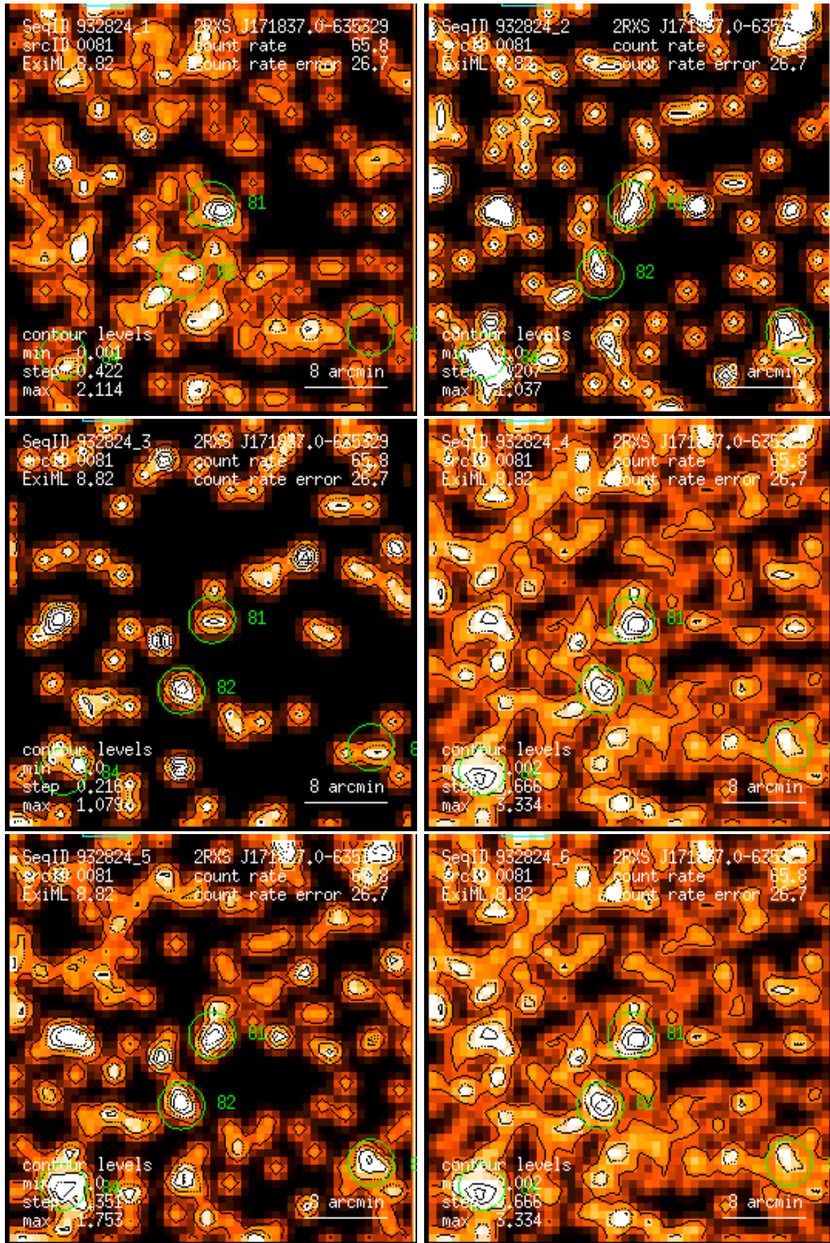
Figure 81: RASS 932824: detection 0081: band rate images, Gaussian filter: (1) PSPC channels 11 – 41, (2) 52 – 90, (3) 91 – 201, (4) 11 – 235, (5) 52 – 201, (6) 11 – 201. Broad band rates in counts/ks. Band rate contour levels in counts/ks/arcmin 2 .
