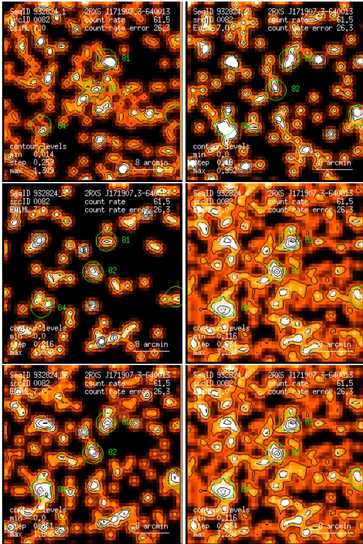
Figure 82: RASS 932824: detection 0082: band rate images, Gaussian filter: (1) PSPC channels 11 – 41, (2) 52 – 90, (3) 91 – 201, (4) 11 – 235, (5) 52 – 201, (6) 11 – 201. Broad band rates in counts/ks. Band rate contour levels in counts/ks/arcmin 2 .
