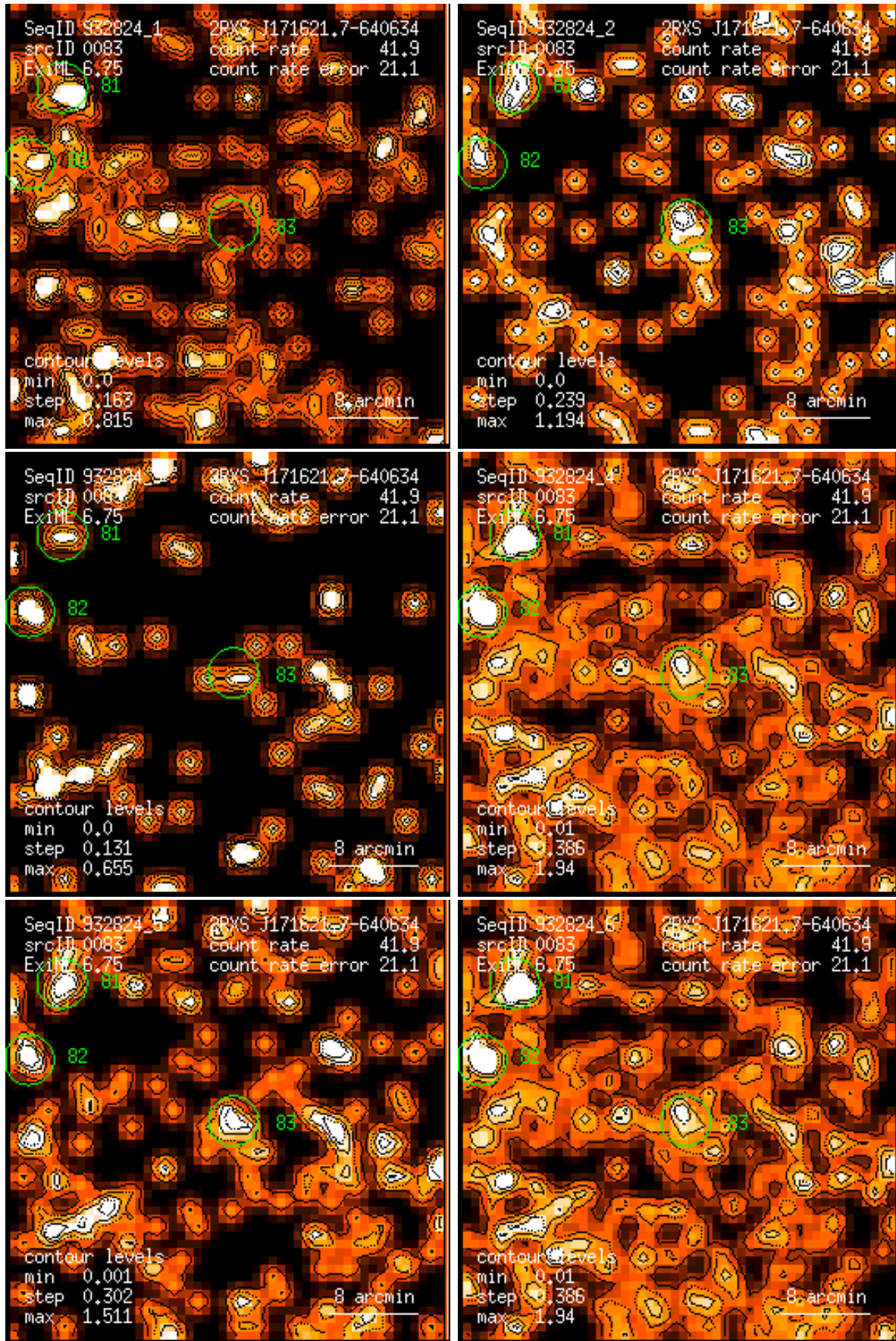
Figure 83: RASS 932824: detection 0083: band rate images, Gaussian filter: (1) PSPC channels 11 – 41, (2) 52 – 90, (3) 91 – 201, (4) 11 – 235, (5) 52 – 201, (6) 11 – 201. Broad band rates in counts/ks. Band rate contour levels in counts/ks/arcmin 2 .
