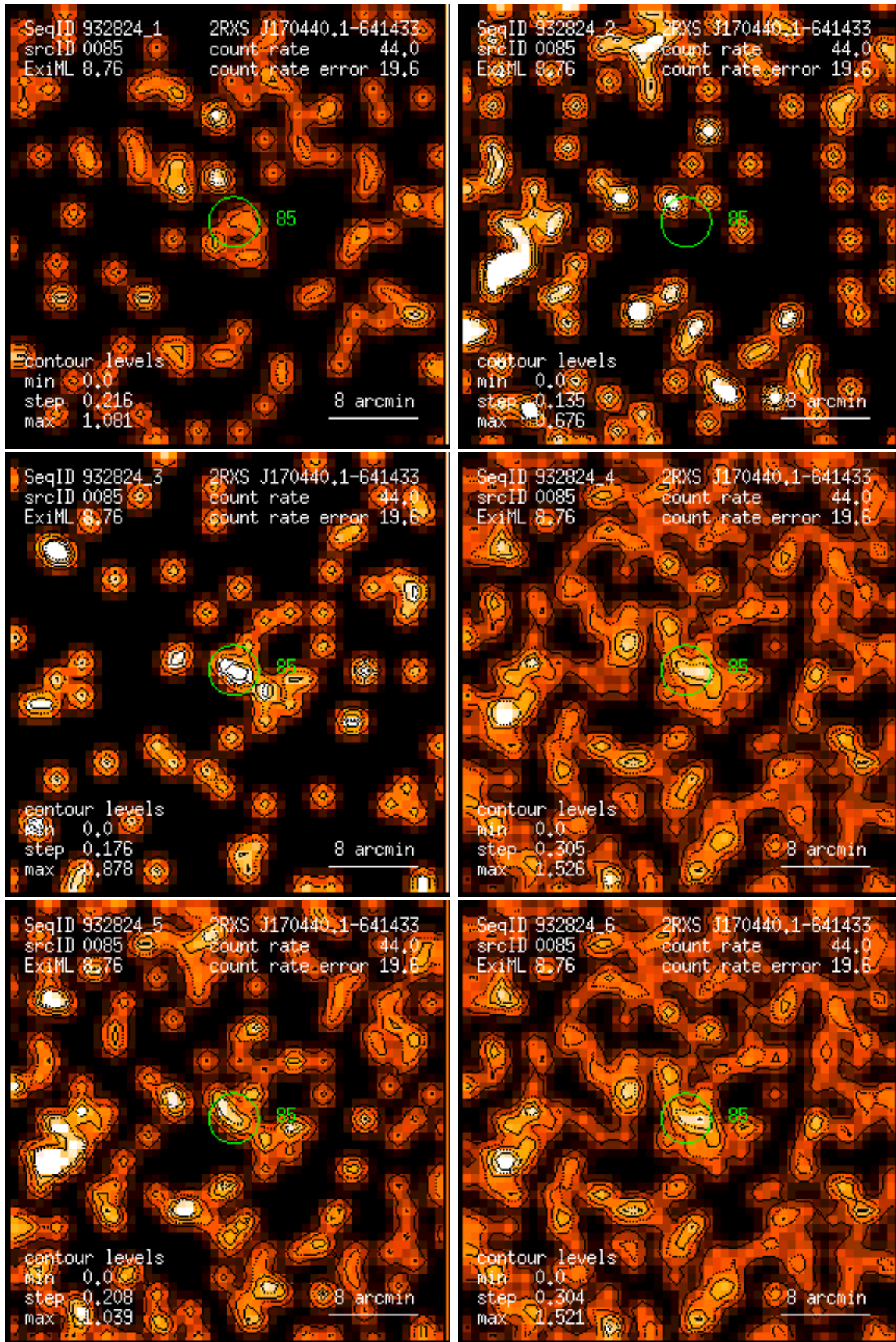
Figure 85: RASS 932824: detection 0085: band rate images, Gaussian filter: (1) PSPC channels 11 – 41, (2) 52 – 90, (3) 91 – 201, (4) 11 – 235, (5) 52 – 201, (6) 11 – 201. Broad band rates in counts/ks. Band rate contour levels in counts/ks/arcmin 2 .
