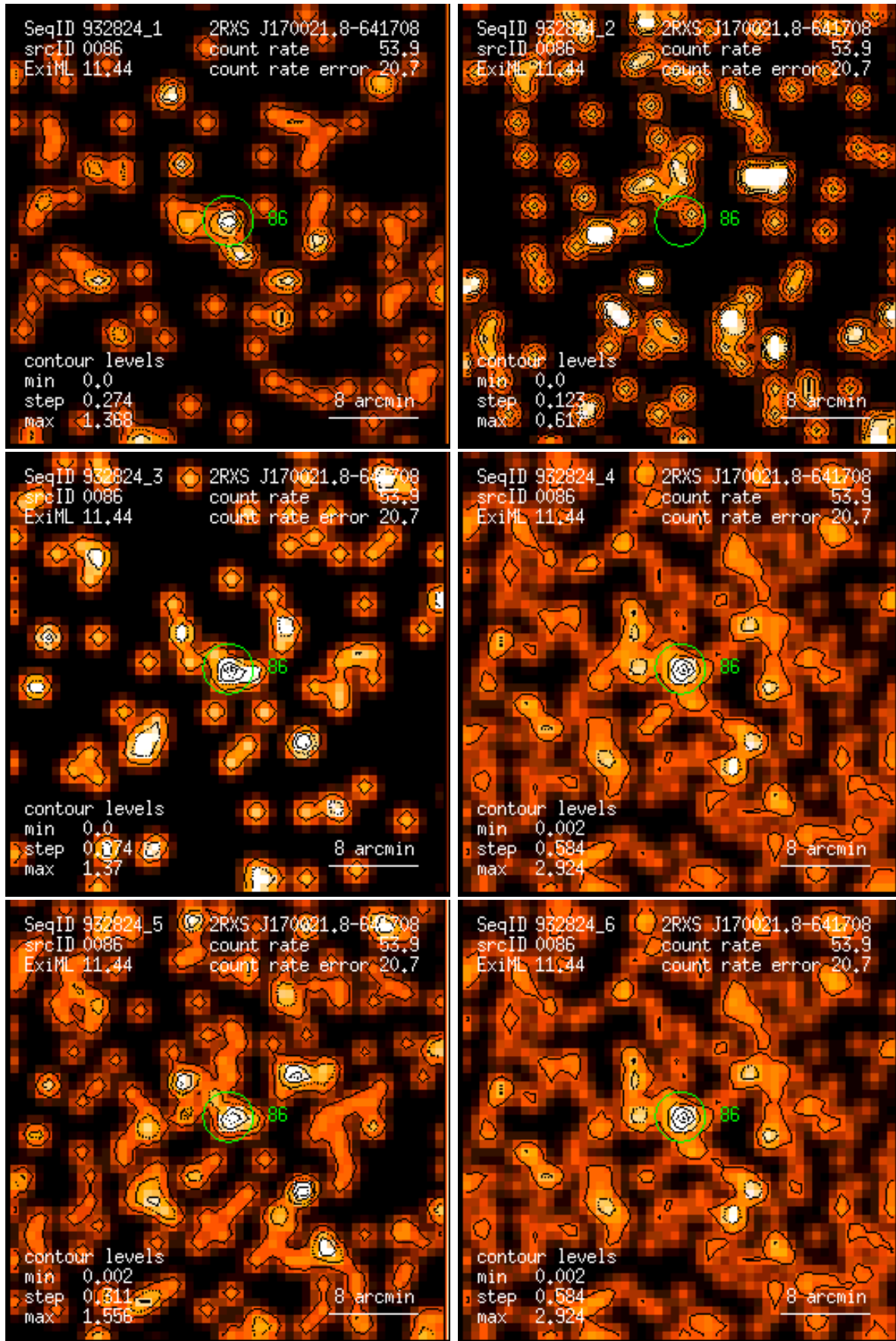
Figure 86: RASS 932824: detection 0086: band rate images, Gaussian filter: (1) PSPC channels 11 – 41, (2) 52 – 90, (3) 91 – 201, (4) 11 – 235, (5) 52 – 201, (6) 11 – 201. Broad band rates in counts/ks. Band rate contour levels in counts/ks/arcmin 2 .
