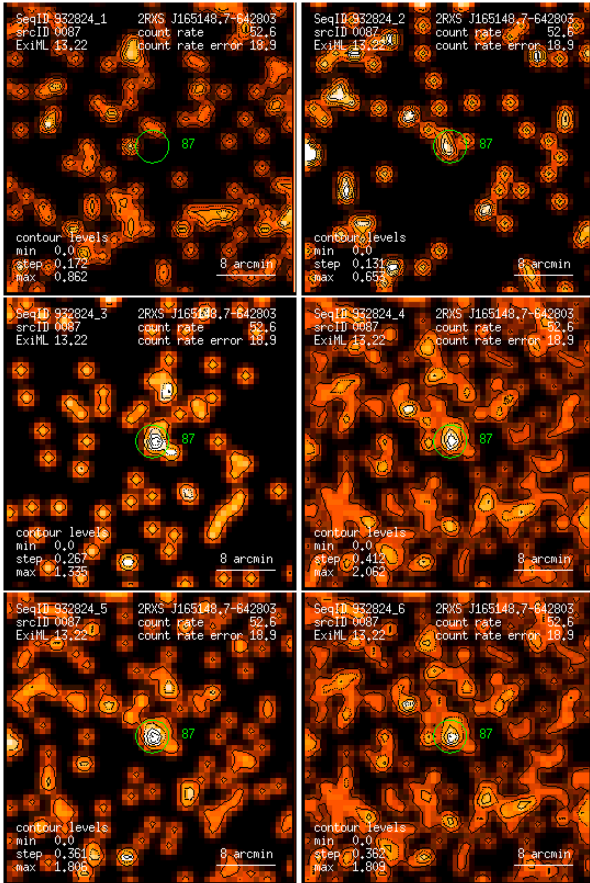
Figure 87: RASS 932824: detection 0087: band rate images, Gaussian filter: (1) PSPC channels 11 – 41, (2) 52 – 90, (3) 91 – 201, (4) 11 – 235, (5) 52 – 201, (6) 11 – 201. Broad band rates in counts/ks. Band rate contour levels in counts/ks/arcmin 2 .
