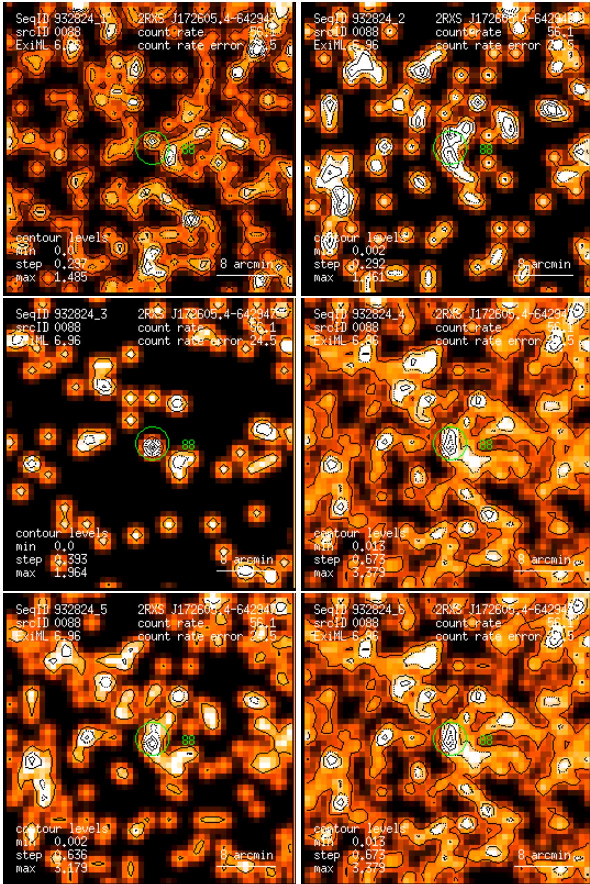
Figure 88: RASS 932824: detection 0088: band rate images, Gaussian filter: (1) PSPC channels 11 – 41, (2) 52 – 90, (3) 91 – 201, (4) 11 – 235, (5) 52 – 201, (6) 11 – 201. Broad band rates in counts/ks. Band rate contour levels in counts/ks/arcmin 2 .
