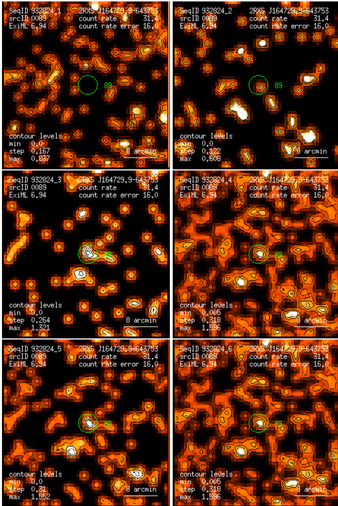
Figure 89: RASS 932824: detection 0089: band rate images, Gaussian filter: (1) PSPC channels 11 – 41, (2) 52 – 90, (3) 91 – 201, (4) 11 – 235, (5) 52 – 201, (6) 11 – 201. Broad band rates in counts/ks. Band rate contour levels in counts/ks/arcmin 2 .
