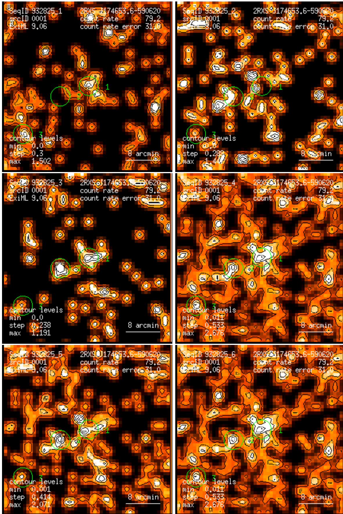
Figure 1: RASS 932825: detection 0001: band rate images, Gaussian filter: (1) PSPC channels 11 – 41, (2) 52 – 90, (3) 91 – 201, (4) 11 – 235, (5) 52 – 201, (6) 11 – 201. Broad band rates in counts/ks. Band rate contour levels in counts/ks/arcmin 2 .
