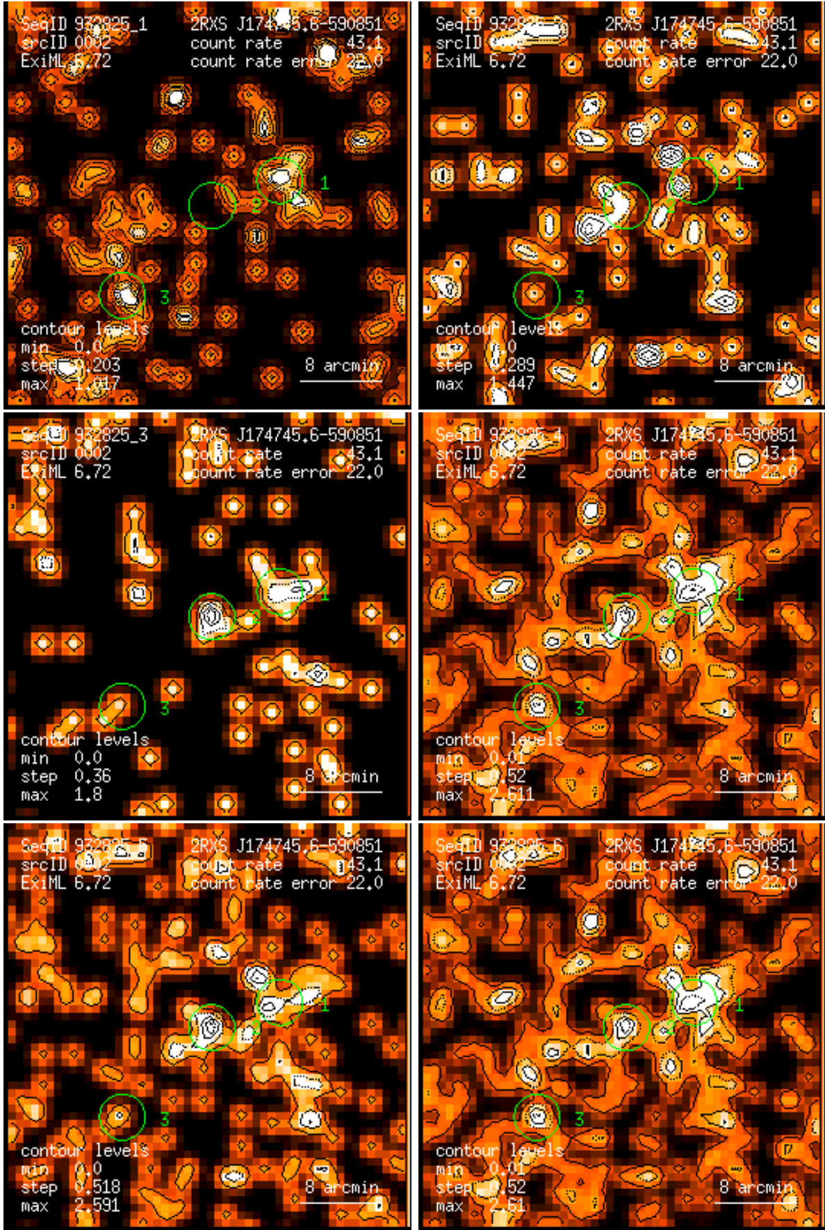
Figure 2: RASS 932825: detection 0002: band rate images, Gaussian filter: (1) PSPC channels 11 – 41, (2) 52 – 90, (3) 91 – 201, (4) 11 – 235, (5) 52 – 201, (6) 11 – 201. Broad band rates in counts/ks. Band rate contour levels in counts/ks/arcmin 2 .
