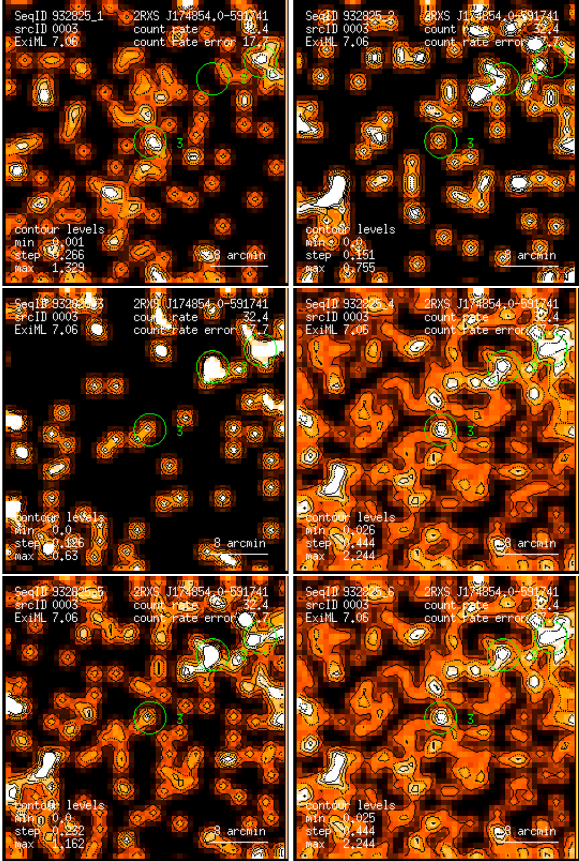
Figure 3: RASS 932825: detection 0003: band rate images, Gaussian filter: (1) PSPC channels 11 – 41, (2) 52 – 90, (3) 91 – 201, (4) 11 – 235, (5) 52 – 201, (6) 11 – 201. Broad band rates in counts/ks. Band rate contour levels in counts/ks/arcmin 2 .
