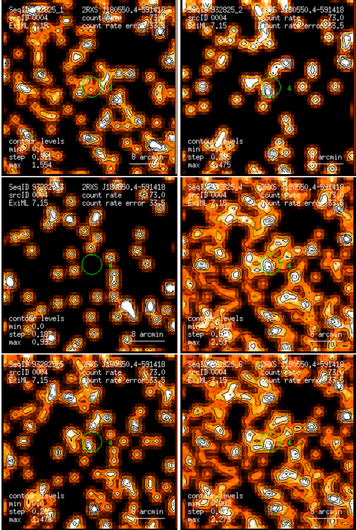
Figure 4: RASS 932825: detection 0004: band rate images, Gaussian filter: (1) PSPC channels 11 – 41, (2) 52 – 90, (3) 91 – 201, (4) 11 – 235, (5) 52 – 201, (6) 11 – 201. Broad band rates in counts/ks. Band rate contour levels in counts/ks/arcmin 2 .
