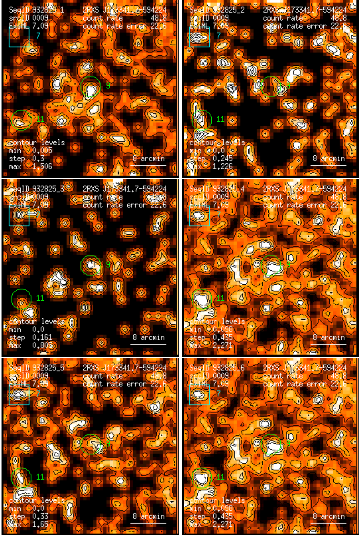
Figure 9: RASS 932825: detection 0009: band rate images, Gaussian filter: (1) PSPC channels 11 – 41, (2) 52 – 90, (3) 91 – 201, (4) 11 – 235, (5) 52 – 201, (6) 11 – 201. Broad band rates in counts/ks. Band rate contour levels in counts/ks/arcmin 2 .
